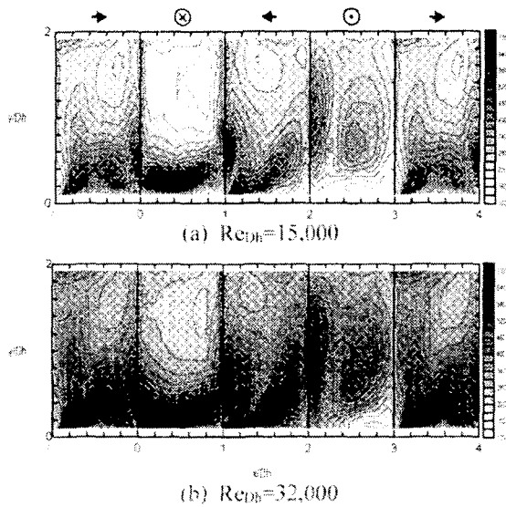
Fig. 8 Contour plots of Sh for different Reynolds number with asymmetric inlet condition at M=0.39
