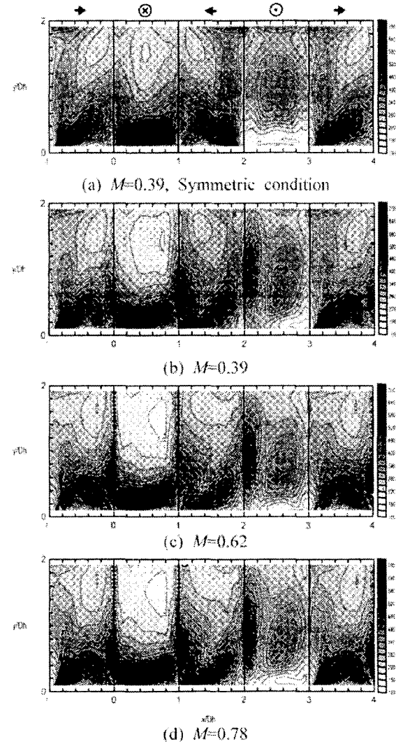
Fig. 5 Contour plots of Sh for various blowing ratios with asymmetric inlet condition at Re_{Dh}=25,000
