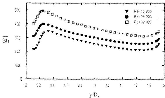
Fig. 9 Average Sherwood number distributions for various Reynolds number with asymmetric inlet condition at M=0.39
