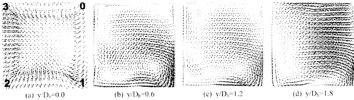
Fig. 2 Velocity vector plots in square film cooling hole with asymmetric inlet condition (not in scale)
