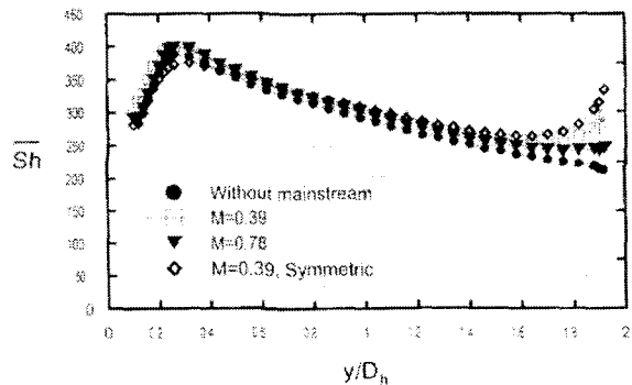
Fig. 7 Average Sherwood number distributions for various blowing ratios with asymmetric inlet condition at Re_{Dh}=25,000
