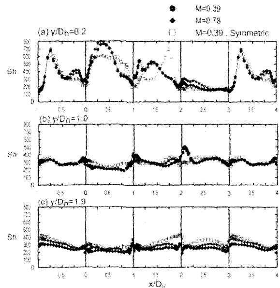
Fig. 6 Local distributions of Sh for various blowing ratios with asymmetric inlet condition at Re_{Dh}=25,000
