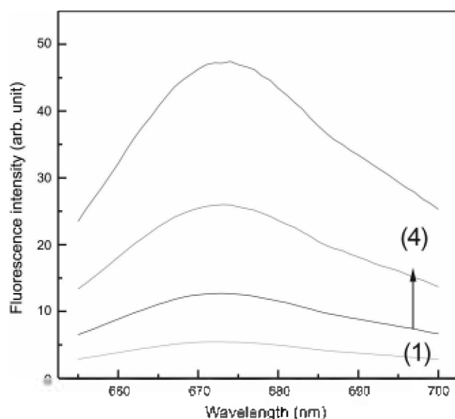
Figure 1. Emission spectra of the Nile Blue-BSA-Triton X-100 system: \lambda_{\text{ex}} = 635 nm; [Nile Blue], 3.3 \times 10^{-5} M; [Triton X-100], 1.5 \times 10^{-3} %; pH 6.8. [BSA]: (1) 1.0; (2) 2.0; (3) 5.0; (4) 10.0 \mu\text{g/mL} .
