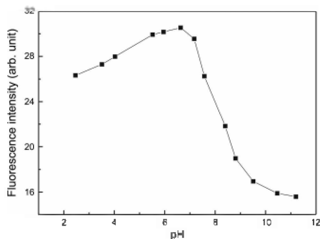
Figure 2. Effect of pH on emission intensity of the Nile Blue-BSA-Triton X-100 system: [Nile Blue], 3.3 \times 10^{-5} M; [Triton X-100], 1.5 \times 10^{-3} %; [BSA], 10.0 \mu\text{g/mL} .
