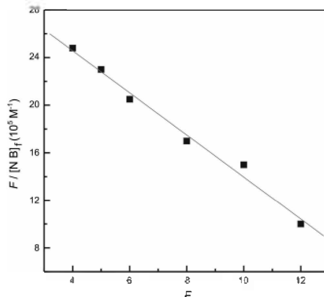
Figure 5. Scatchard plot at pH 6.8.
