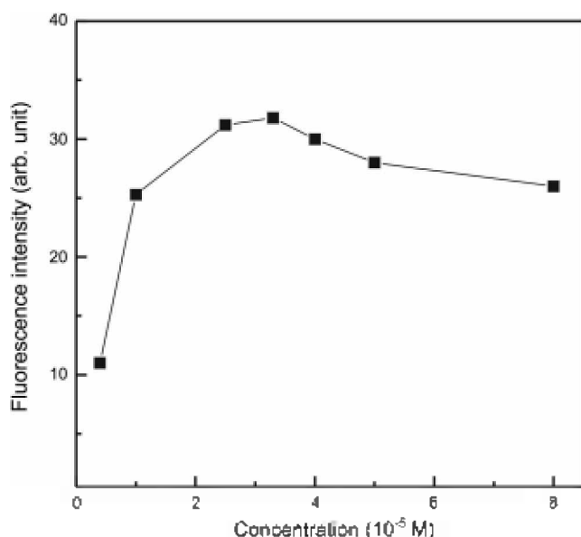
Figure 3. Effect of Nile Blue concentration on emission intensity of the Nile Blue-BSA-Triton X-100 system: [Triton X-100], 2.0 \times 10^{-3} %; [BSA], 10.0 \mu\text{g/mL} ; pH 6.8.
