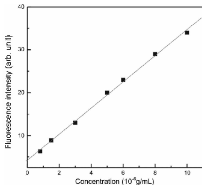
Figure 6. Calibration curve for BSA standard solution: [Nile Blue], 3.3 \times 10^{-5} M; [Triton X-100], 1.5 \times 10^{-3} %; pH 6.8.
