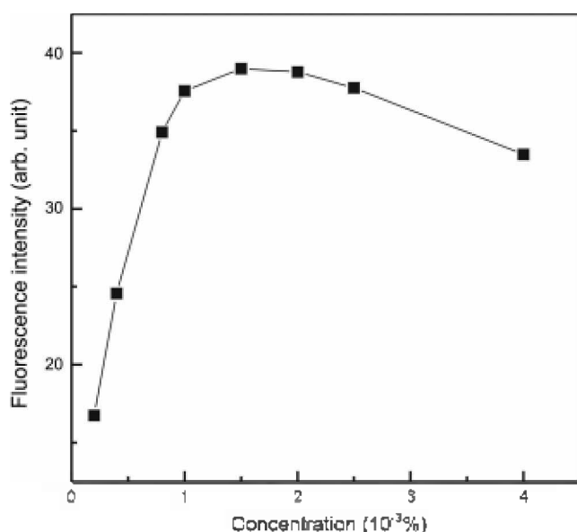
Figure 4. Effect of Triton X-100 concentration on emission intensity of the BSA-Nile Blue system: [Nile Blue], 3.3 \times 10^{-5} M; [BSA], 10.0 \mu\text{g/mL} ; pH 6.8.
