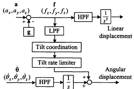
Fig. 8 Block diagram of classical washout algorithm
