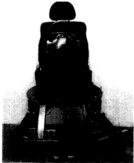
Fig. 1 Photo of motion simulator KU-MS
