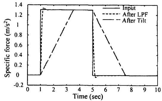
Fig. 14 Specific force by tilt coordination with no fuzzy logic
