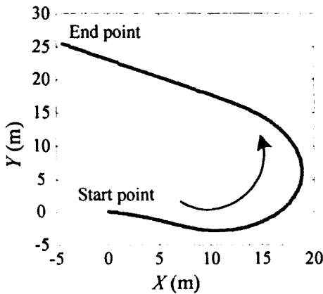
Fig. 6 Bicycle trajectory by joystick input
