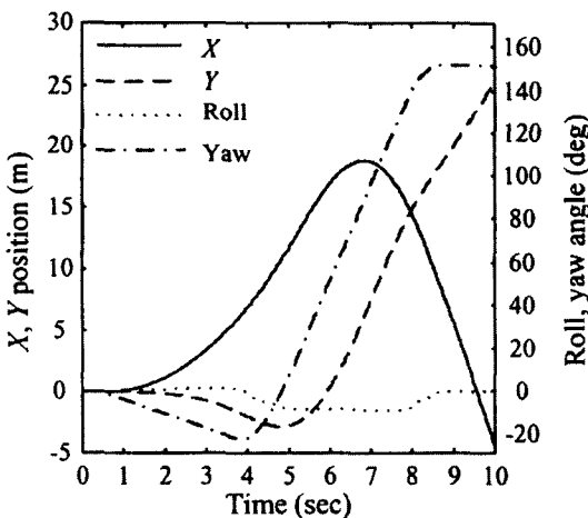
Fig. 7 Bicycle position and orientation by joystick input
