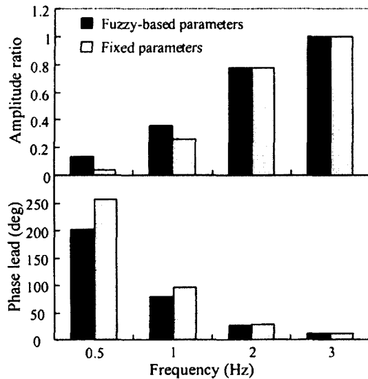
Fig. 13 Amplitude ratios and phase leads of fuzzy-based and fixed parameters
