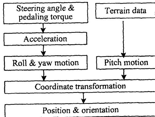
Fig. 5 Flow chart for bicycle dynamics
