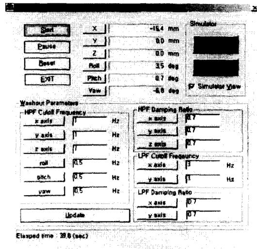
Fig. 9 Control panel of motion base
