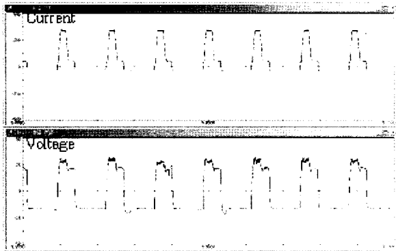
Fig. 12 Waveform at EN ratio 40% in polarity control AC pulse MIG welding(Current 60A)
