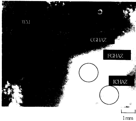
Fig. 1 Macroetched weldment
