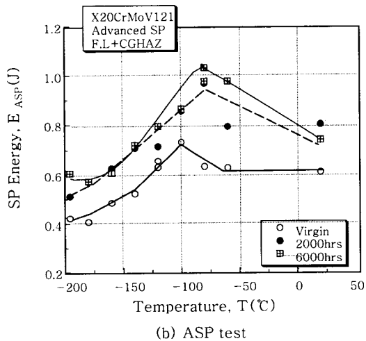
Fig. 9 SP energy transitions behavior with aging times for F.L+CGHAZ in SP test
