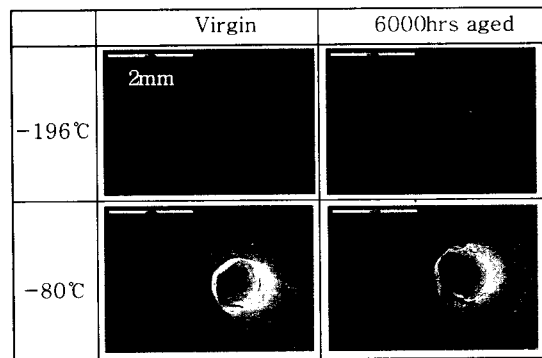
(a) Macro fractographs
