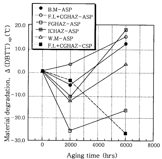
Fig. 8 Variation of \Delta(\text{DBTT})_{SP} according to aging times in ASP & CSP test
