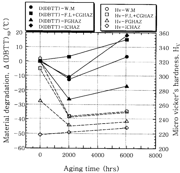
Fig. 11 Relationships between \Delta(DBTT)_{ASP} and micro-Vicker's hardness
