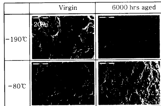
(b) Micro fractographs
