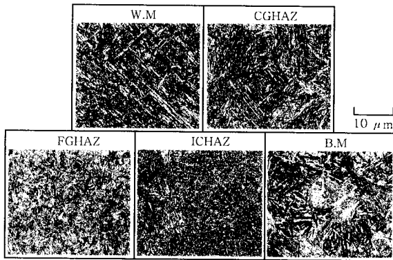
Fig. 2 Microstructures of virgin weldment
