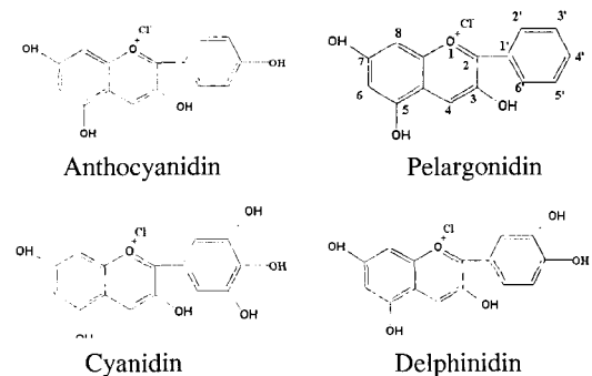
Scheme 1. The structure of the principal ingredient of Anthocyanins.
