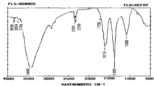
Fig. 6. FT-IR spectrum of Impatiens balsamina blossom extracts with water.
