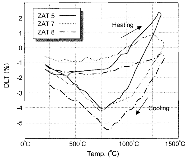
Fig. 3. Thermal expansion curves of ZAT composites sintered at 1600°C for 2 h.
