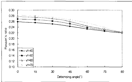
Fig. 5 The effect of fiber volume fraction( V_f ) on the composite Poisson's ratio \nu_{31} .
