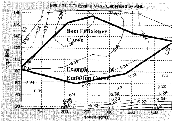
Figure 2. MB 1.7L Engine Map (ANL data).
