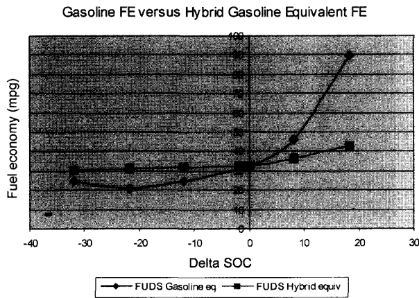
Figure 7. Fuel economy correction for SOC.
