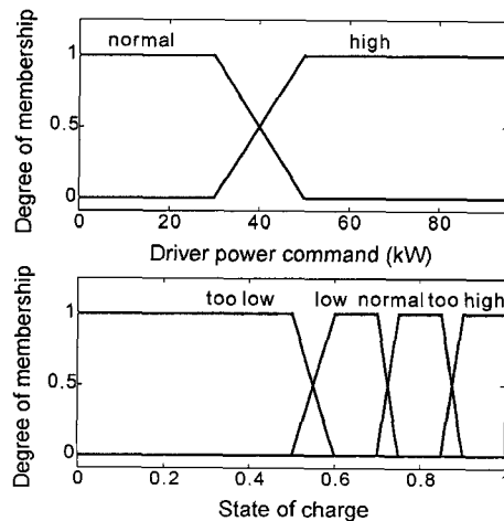
Figure 4. Example of membership functions.
