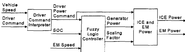
Figure 3. Fuzzy logic controller block diagram.
