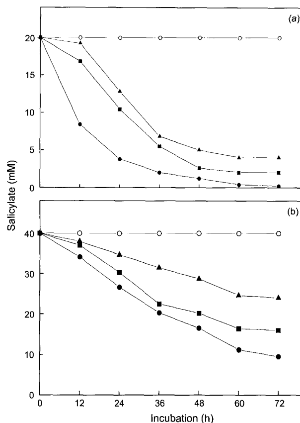
Fig. 1. Degradation of salicylate in batches with (a) 20 mM and (b) 40 mM.
