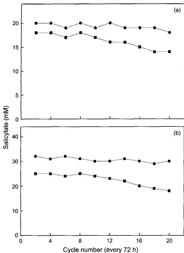
Fig. 2. Semi-continuous degradation of salicylate at 20 mM (a) and 40 mM (b). (■) and (●) are alginate ( 3.2 \times 10^{11} cfu·g -1 ) and polyurethane foam ( 3 \times 10^{11} cfu·g -1 ) immobilized cell systems, respectively.
