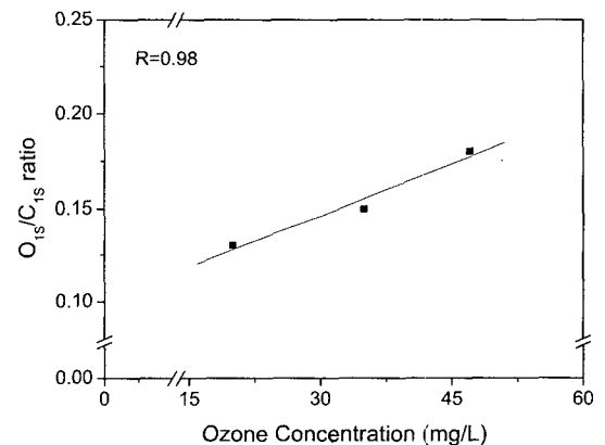
Figure 10. Dependence of O 1s /C 1s ratio with (a) total transferred ozone amount and (b) O 3 concentration (R = coefficient of regression).
