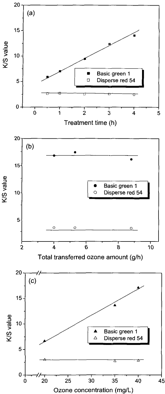
Figure 11. Relationship between K/S value and ozone treated LDPE film dyed with C. I. Disperse Red 54 and C. I. Green 1 (a; ozone treatment time, b; total transferred ozone amount, c; ozone concentration).
