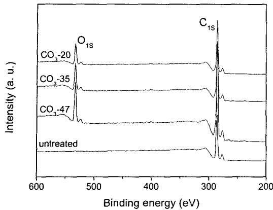
Figure 8. XPS survey scan spectra as a function of ozone concentration.
