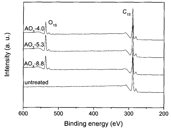
Figure 6. XPS survey scan spectra as a function of total transferred ozone amount.
