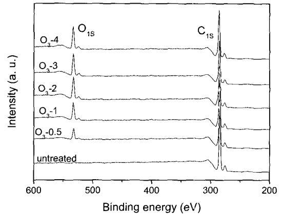
Figure 2. XPS survey scan spectra as a function of ozone treatment time.
