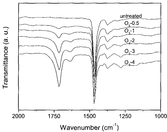
Figure 1. FTIR-ATR spectra as a function of ozone treatment time.
