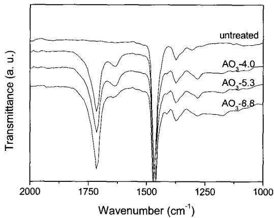
Figure 5. FTIR-ATR spectra as a function of total transferred ozone amount.
