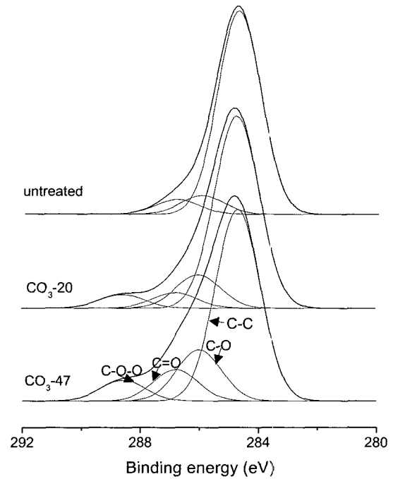
Figure 9. C 1s XPS spectra as a function of ozone concentration.
