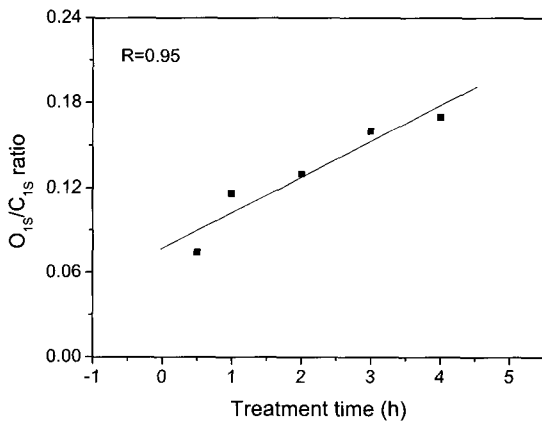
Figure 4. Dependence of O 1s /C 1s ratio with ozone treatment time (R = coefficient of regression).
