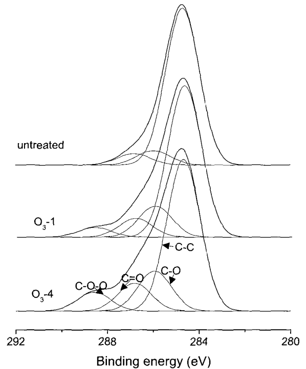
Figure 3. C 1s XPS spectra as a function of ozone treatment time.
