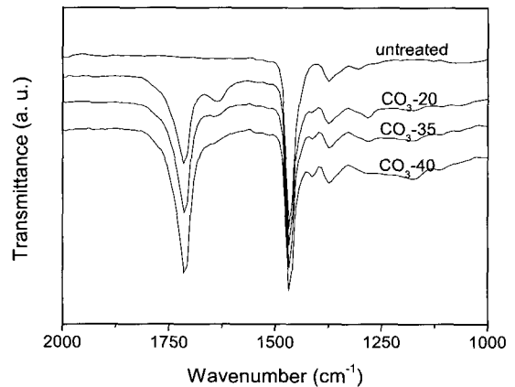
Figure 7. FTIR-ATR spectra as a function of ozone concentration.
