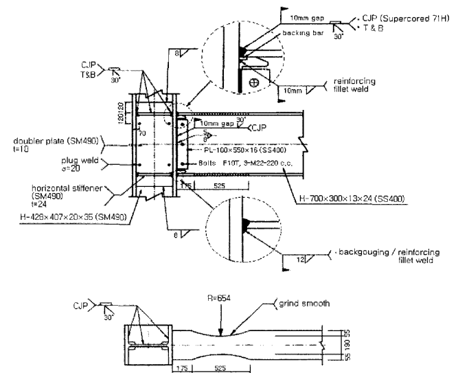
Fig. 3 Specimen DB700-SW moment connection details
