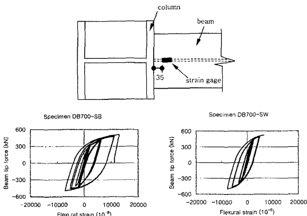
Fig. 14 Comparison of flexural strain responses near groove weld up to the fracture of specimen DB700-SB
