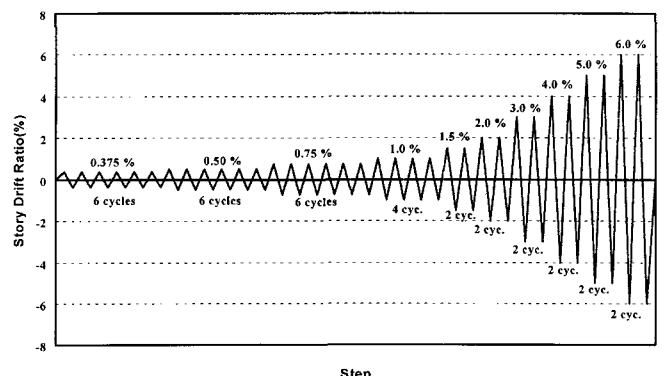
Fig. 6 SAC 2000 standard loading history
