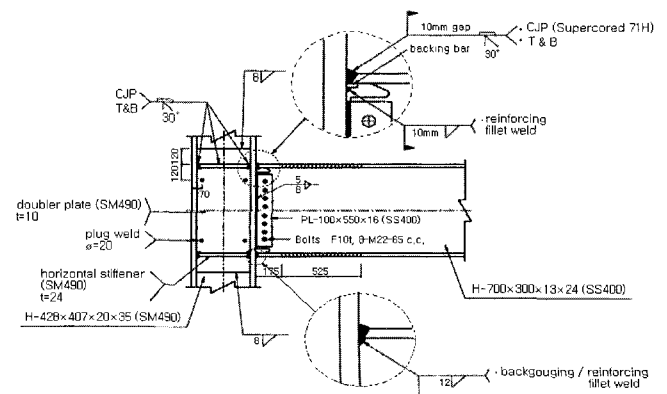
Fig. 4 Specimen DB700-SB moment connection details
