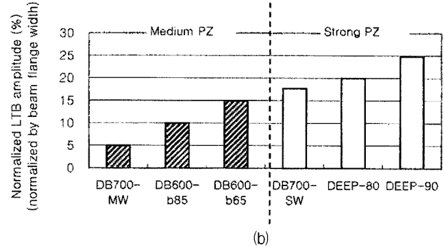
Fig. 19 Comparison of the measured LTB amplitudes at the 4% story drift
