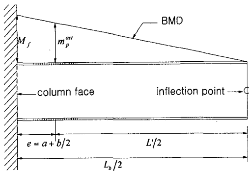
Fig. 1 Typical geometry of the radius cut RBS
