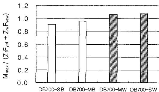
Fig. 12 Comparison of connection strength(set #1)
