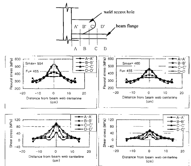
Fig. 13 Analytical stress distribution around weld access hole at fracture load (specimen DB700-SB): (a) assuming that the beam web is totally inactive, (b) assuming that the beam web is fully active
