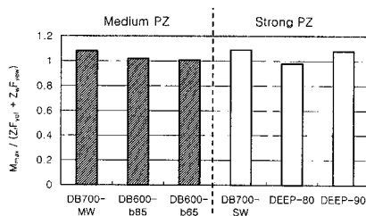
Fig. 18 Comparison of connection strength (medium versus strong panel zone)
