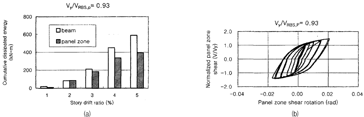
Fig. 21 Cumulative energy dissipation and cyclic shear response of the panel zone(DB700-MW)
