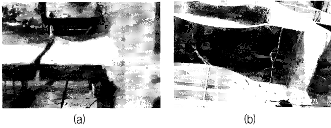
Fig. 8 Beam bottom flange fracture of specimen DB700-SB at 2% story drift cycle
