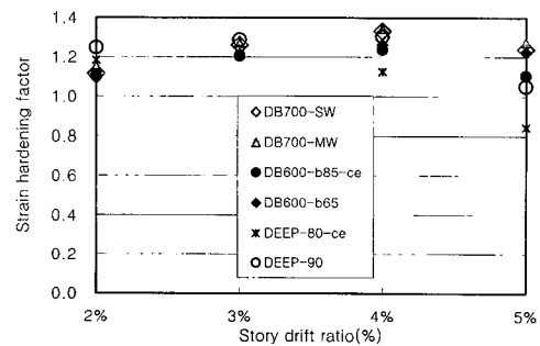
Fig. 20 Story drift ratio versus strain hardening factors
