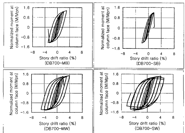
Fig. 7 Normalized moment versus story drift ratio relationship(test set #1)
