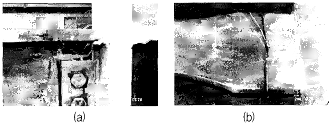
Fig. 9 Beam top flange fracture of specimen DB700-MB at 3% story drift cycle
