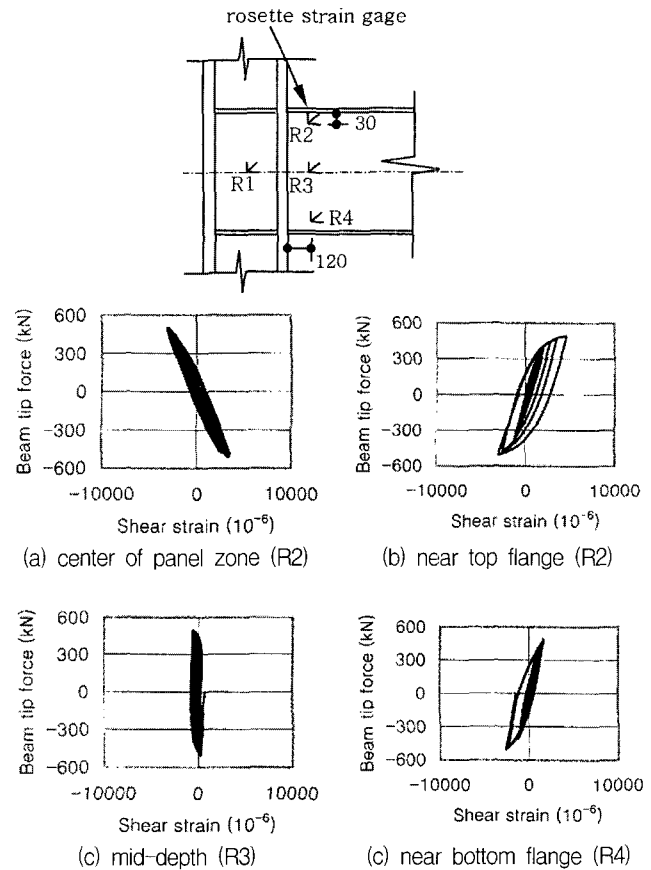
Fig. 15 Measured cyclic shear strain responses(specimen DB700-SB)
