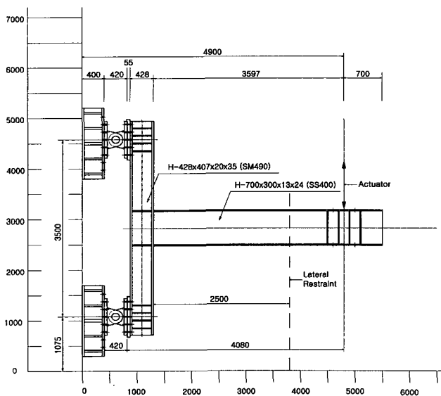
Fig. 5 Typical test setup
