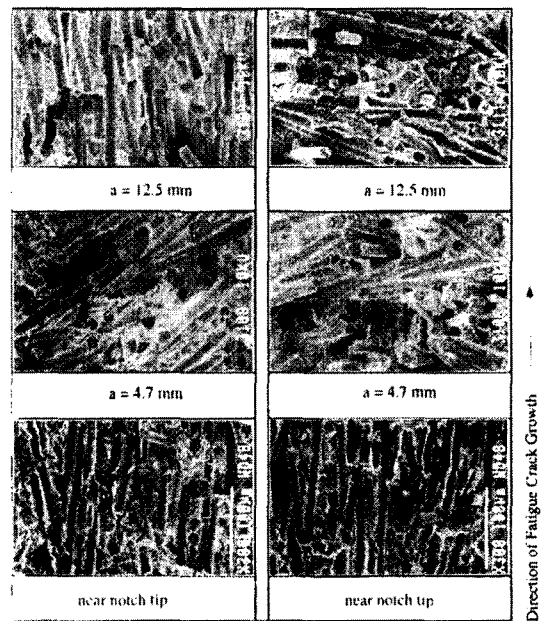
Fig. 10 Variation of fracture surface along the crack growth of PPS weld (TW)
