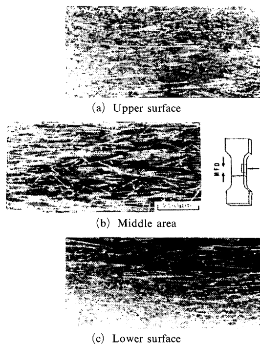
Fig. 3 Photomicrographs taken on fiber orientation in the parallel plane of injection molded PPS parent.
