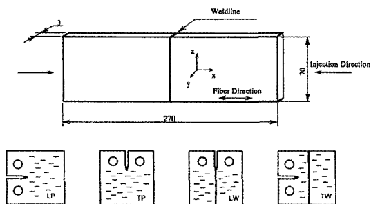
Fig. 2 Layout and dimensions of injection mold and extraction of CT specimen
