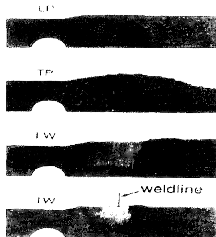
Fig. 6 Configuration of fatigue crack growth at PPS parent and weld
