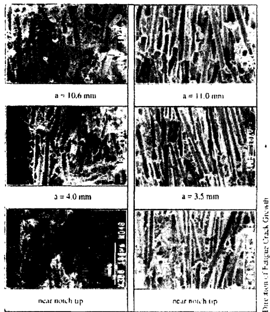
Fig. 8 Variation of fracture surface along the crack growth of PPS parent (TP)
