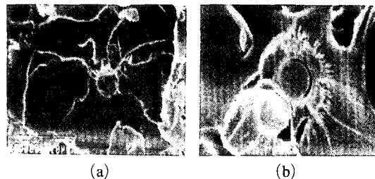
Fig. 14 Fatigue crack initiation and propagation at fiber parallel to the loading direction (a) crack growth behavior due to precrack of fiber (b) energy accumulation and hardening around fiber
