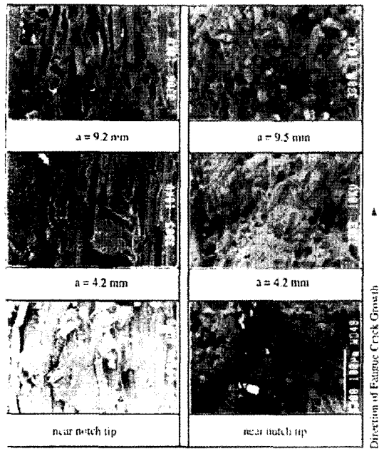
Fig. 7 Variation of fracture surface along the crack growth of PPS parent (LP)
