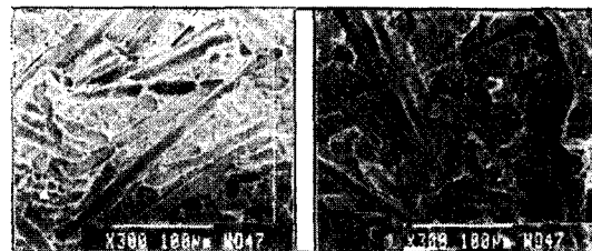
Fig. 12 Fractography of PPS weld after fatigue testing
