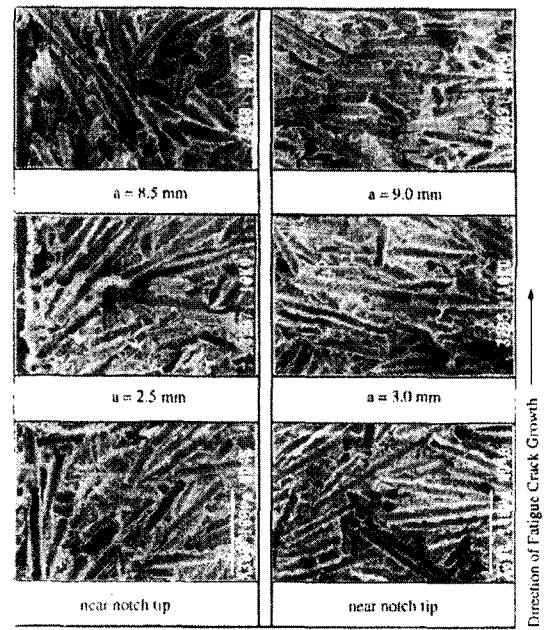
Fig. 9 Variation of fracture surface along the crack growth of PPS weld (LW)
