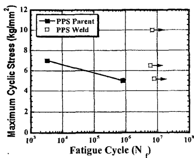
Fig. 11 Relation between maximum cyclic stress and fatigue cycle of PPS
