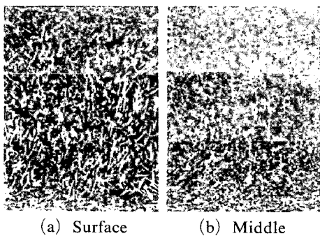
Fig. 5 Photomicrographs of volcano-like pattern of PPS weld magnified in y-z plane.
