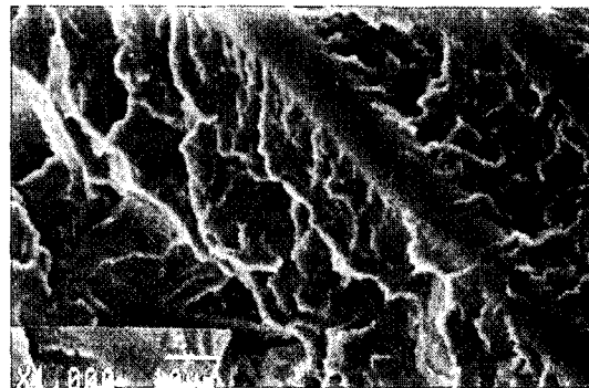
Fig. 13 Fatigue crack initiation and propagation of PPS weld at interface of fiber and matrix
