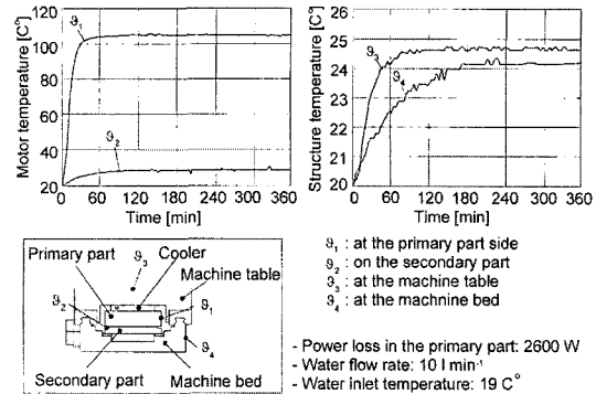
Fig. 4 Temperature measured with the linear motor
