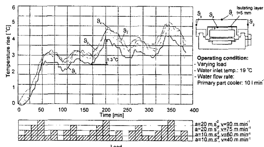
(b) Temperature fluctuation in the machine table with insulation layer
