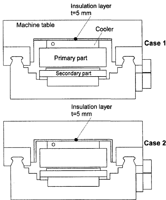
Fig. 7 Arrangements of the insulation layer
