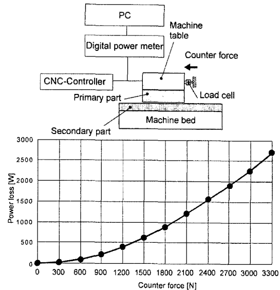
Fig. 2 Electrical power loss of linear motor in dependence on the force
