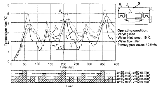
(a) Temperature fluctuation in the machine table without insulation layer
