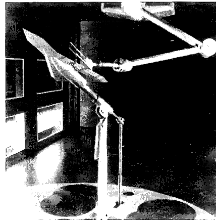
Fig. 1 LEX/Delta wing model in the test section of the KAFA subsonic wind tunnel
