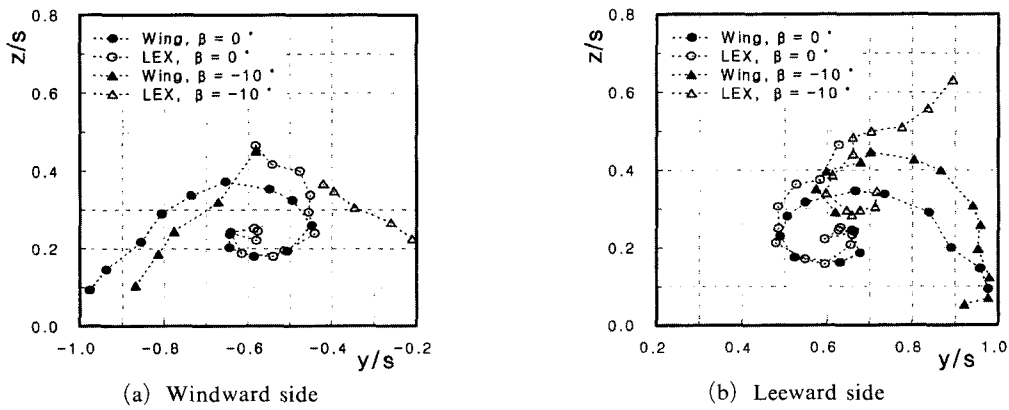
Fig. 5 Locus of vortex cores at different chord station ( \alpha=24^\circ, \beta=-10^\circ )
