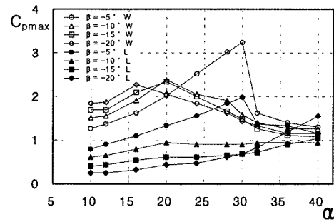
(b) x/c = 0.43
