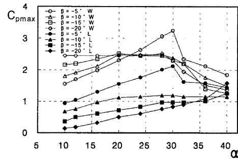
(a) x/c = 0.3
