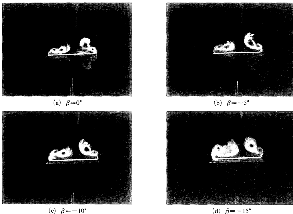
Fig. 7 Effect of angle of attack on the vortex structure at \beta=-5^\circ , and x/c=0.43
