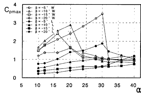
(c) x/c = 0.6
