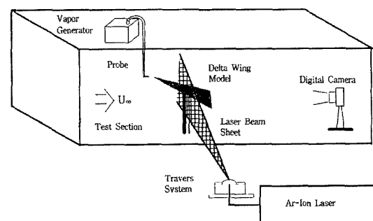
Fig. 3 Experimental set-up for off-surface visualization
