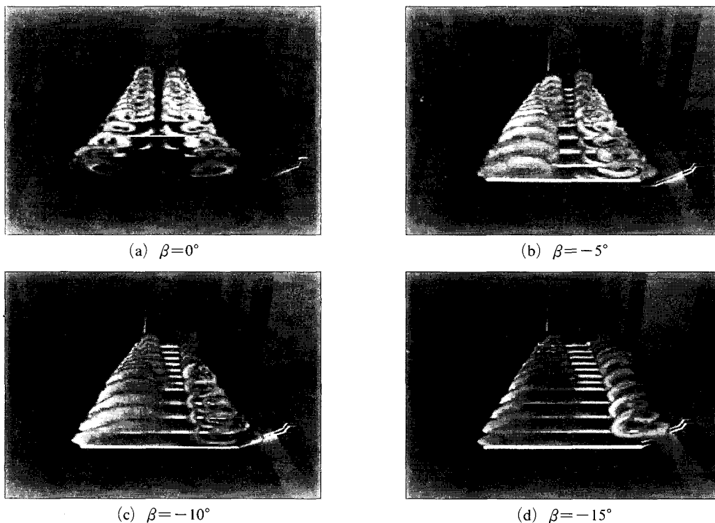
Fig. 4 Perspective photos of the wake section at \alpha=24^\circ
