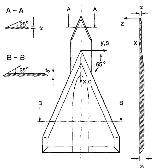
Fig. 2 Geometry of experimental model
