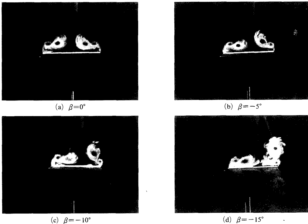
Fig. 6 Effect of sideslip angle on the vortex structure at \alpha=24^\circ , and x/c=0.43
