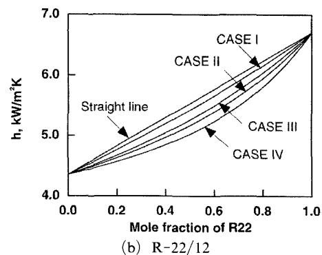
Fig. 4 Predicted heat transfer coefficients for binary refrigerant mixtures with respect to composition for G = 300 \text{ kg/m}^2\text{s} , P = 300 \text{ kPa} , x = 0.7 , and tube diameter = 10 mm
