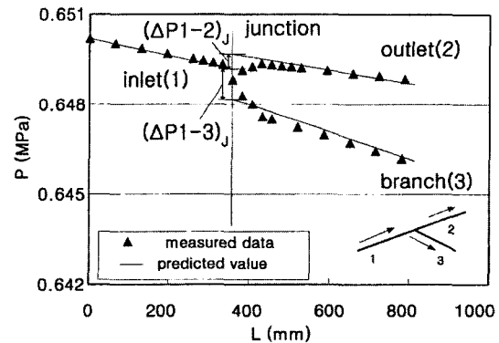
Fig. 3 Pressure profile in the test section for the case HH(I) ( G_1=300 \text{ kg/m}^2\text{s} , x_1=0.3 )
