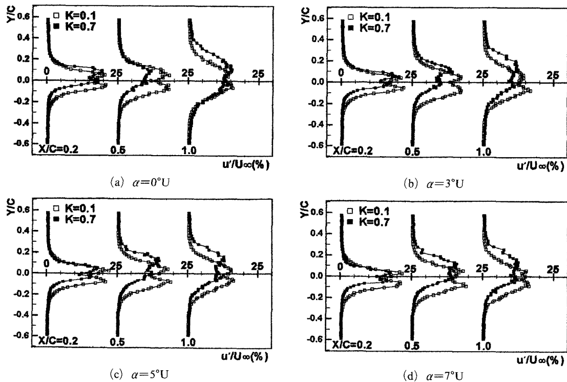
Fig. 6 Trblence intensity profiles during the pitch up motion
