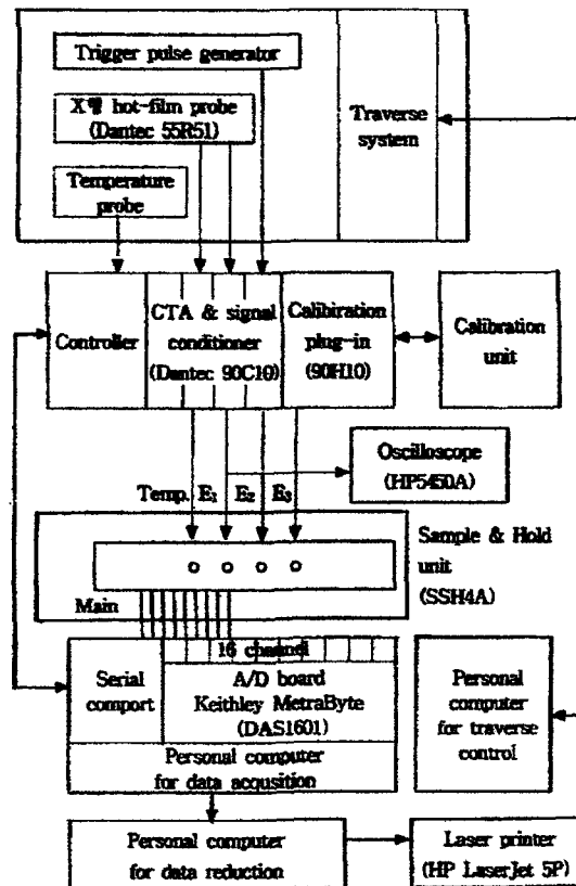
Fig. 2 Block diagram of data acquisition system
