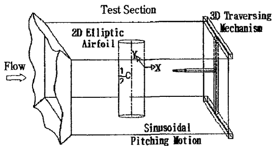
Fig. 1 Schematic of test set-up in test section
