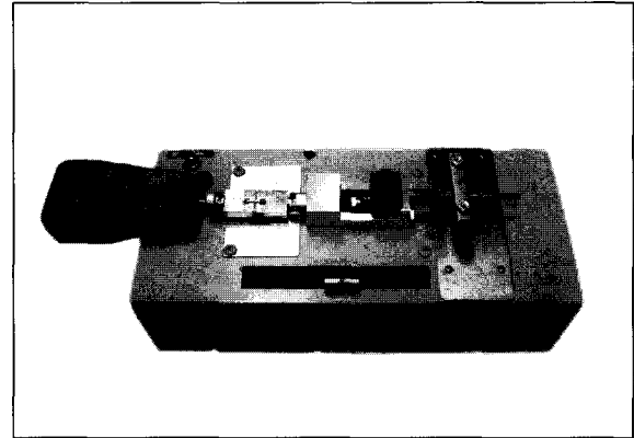
Fig. 6. Microtensile bond strength tester.
