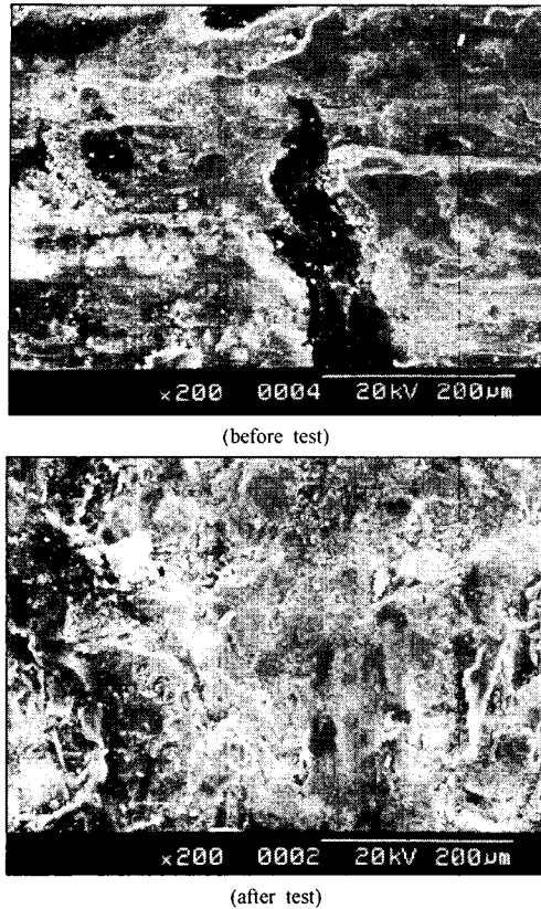
Fig. 11 SEM photographs of AL alloy disk(before and after test).
