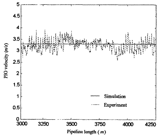
Fig. 8 Simulation and experimental results from 3 km to 4.25 km
