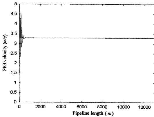
Fig. 6 Simulation velocity of the PIG in the pipeline, 13 km length
