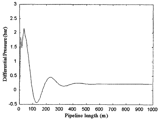
Fig. 5 Differential pressure of the PIG in the inlet pipeline
