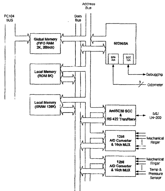
Fig. 4 Schematic diagram of DAU
