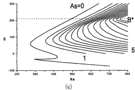
Fig. 4 Spatial amplification contours for moving disturbances at (a) \epsilon=12.5^\circ , (b) 13.3^\circ , and (c) 15^\circ in the Re-B plane
