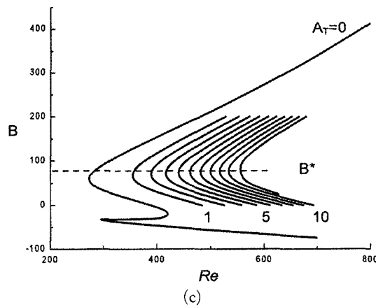
Fig. 5 Temporal amplification contours for (a) \epsilon=12^\circ (b) \epsilon=13.3^\circ and (c) \epsilon=15^\circ in the (Re, B) -planes
