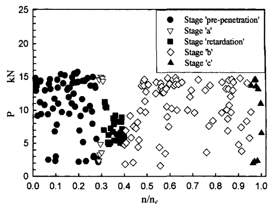
Fig. 6 Relationship between load and normalized signals at different stages of crack growth from specimen AT2
