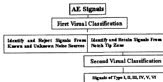
Fig. 7 Flow chart of the visual classification of AE signals
