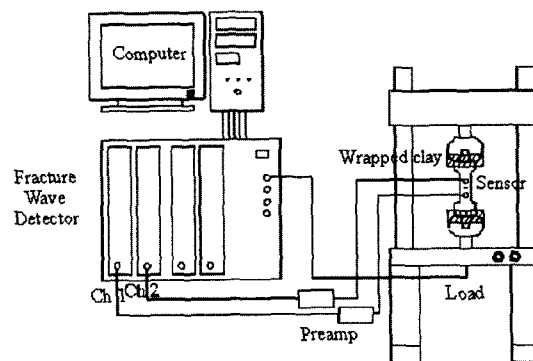
Fig. 2 Measurement system of AE signals
