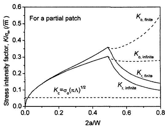
Fig. 4 Stress intensity factor for a partially patched center crack
