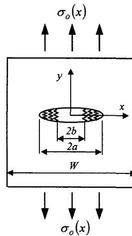
Fig. 2 Distributed springs model for a partially patched crack
