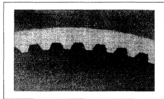
Fig. 3 Enlarged cross-sectional view of internal grooves (60 grooves)
