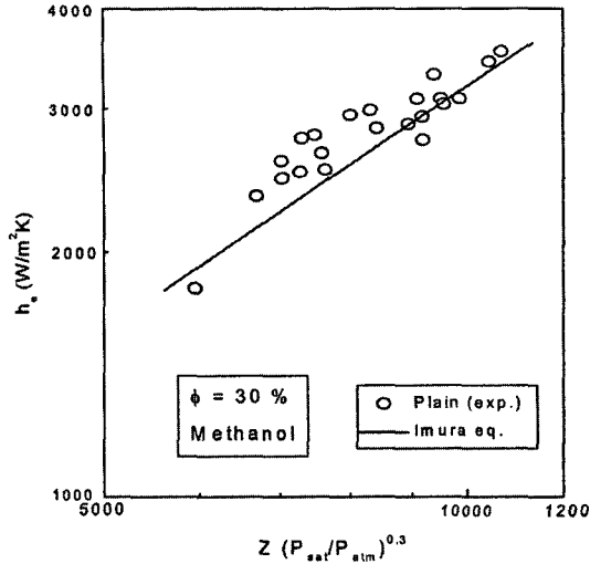
Fig. 5 Comparison of the experimental data with correlations by Imura's equation
