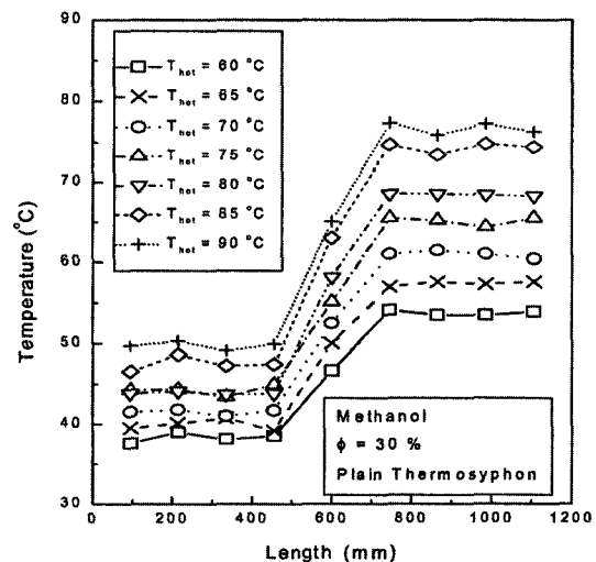
Fig. 4 Temperature distribution along the length of plain thermosyphon
