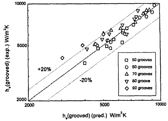
Fig. 8 Comparison of the experimental results with equation (5)
