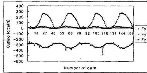
(a) B type(30°+27°), 300rpm of spindle speed
