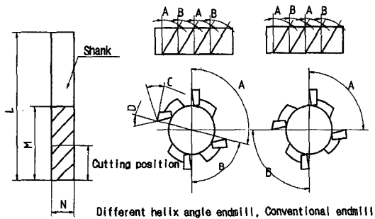
Fig. 4 Schematic diagram of different helix angle endmill
