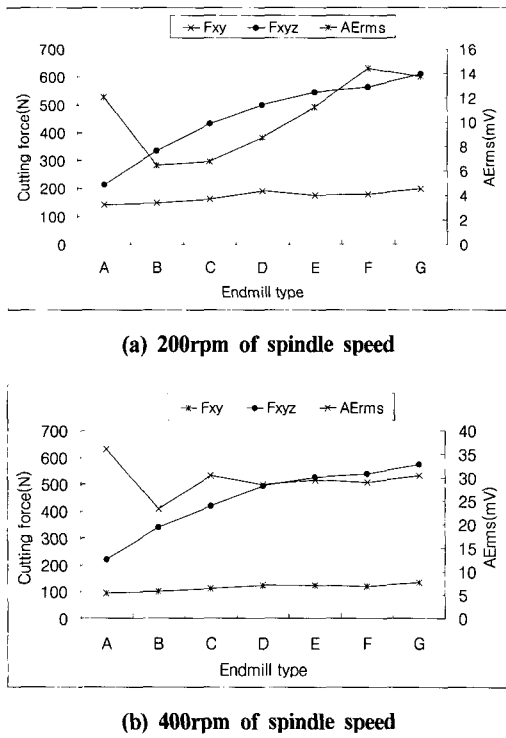
Fig. 6 Relation between AE and cutting force signals according to the change of helix angle for down-cutting
