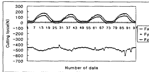
(b) D type(30°+30°), 500rpm of spindle speed
