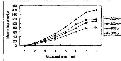
(b) D type endmill(30°+30°)
