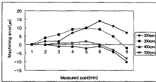
(a) B type endmill (30°+27°)
