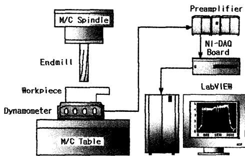
Fig. 2 Diagram of experimental setup
