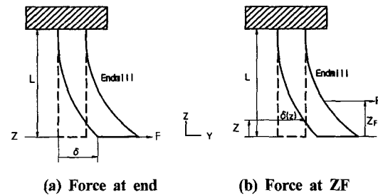
Fig. 1 Tool deflection models
