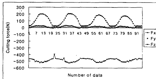
(b) D type(30°+30°), 500rpm of spindle speed
