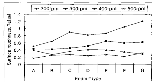
Fig. 11 Surface roughness(Ra) for up-cutting
