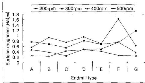
Fig. 12 Surface roughness(Ra) for down-cutting
