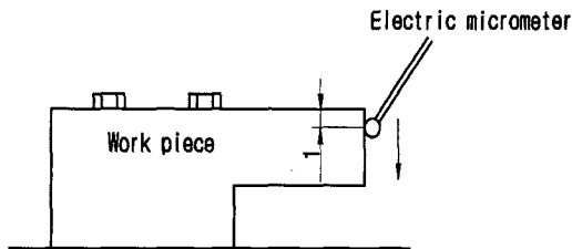
Fig. 3 Measuring method for machining error
