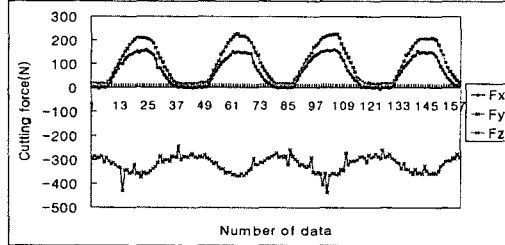
(a) B type(30°+27°), 300rpm of spindle speed
