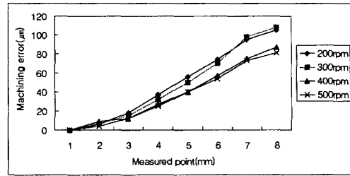
(a) B type endmill(30°+27°)
