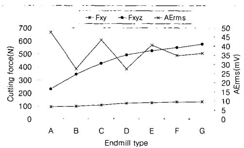
(b) 400rpm of spindle speed
