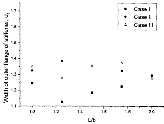
Fig. 8 Width of outer flange of stiffener, d_1 for various aspect ratios
