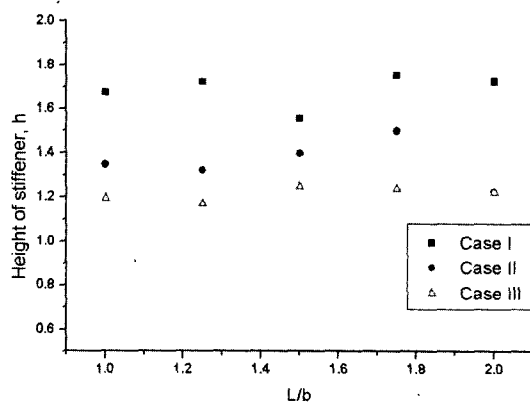
Fig. 9 Height of stiffener, h for various aspect ratios
