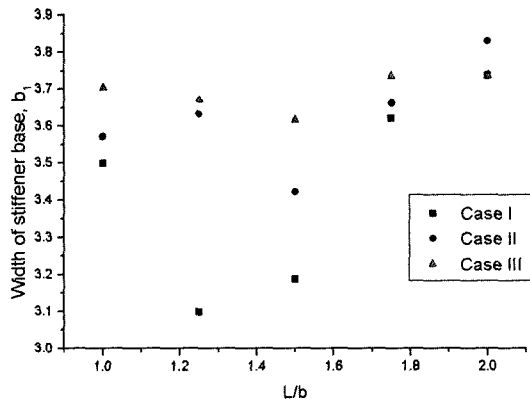
Fig. 6 Width of stiffener base, b_1 for various aspect ratios
