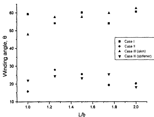
Fig. 4 Winding angle, \theta for various aspect ratios
