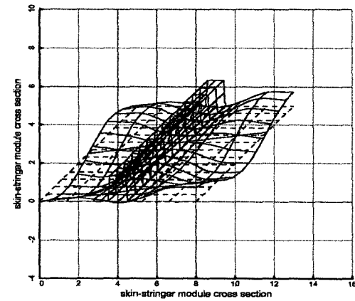
Fig. 11 Local buckling mode shape for single panel module
