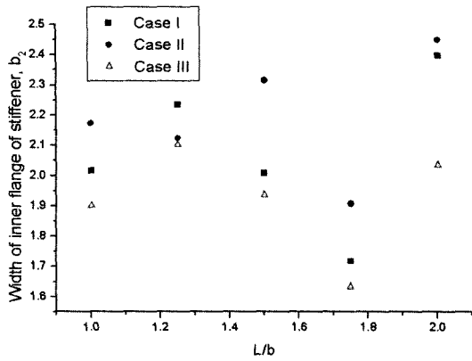
Fig. 7 Width of inner flange of stiffener, b_2 for various aspect ratios
