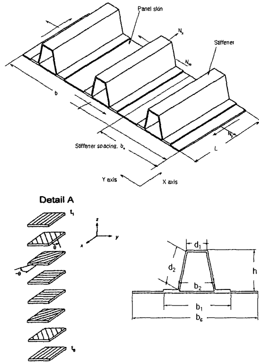
Fig. 1 Stiffened laminated composite panel with trapezoidal type stiffeners
