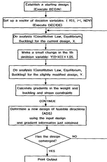
Fig. 2 Flow diagram of optimal design
