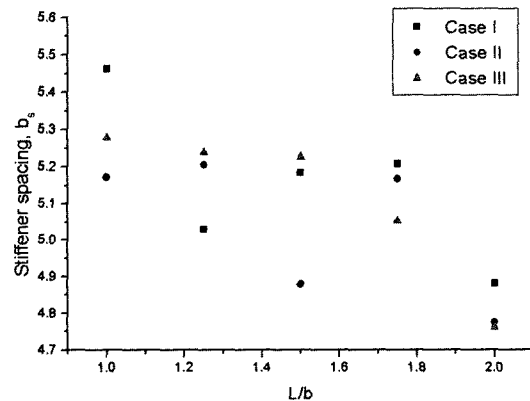
Fig. 5 Stiffener spacing, bs for various aspect ratios
