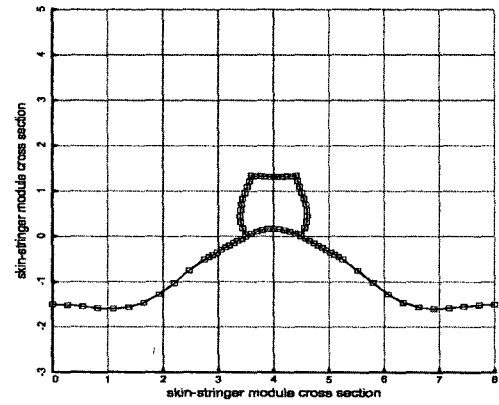
Fig. 10 Wide column buckling mode shape for single panel module
