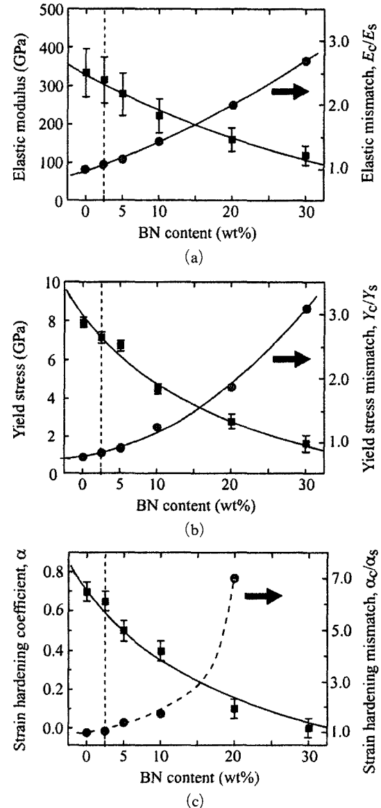
Fig. 4 Elastic and plastic properties of \text{Si}_3\text{N}_4 and \text{Si}_3\text{N}_4 + \text{BN} composites as a function of BN content: (a) elastic modulus, (b) yield stress, and (c) strain hardening coefficient. Elastic/plastic mismatch was inserted in each graph. The data on the dotted lines indicate the data of hard \text{Si}_3\text{N}_4 on soft \text{Si}_3\text{N}_4 .
