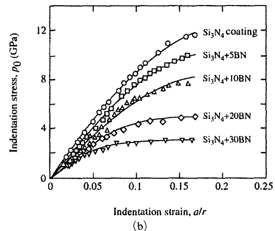
Fig. 3 Indentation stress-strain curves for each layer material used in (a) hard \text{Si}_3\text{N}_4 on soft \text{Si}_3\text{N}_4 and (b) \text{Si}_3\text{N}_4 on \text{Si}_3\text{N}_4+\text{BN}
