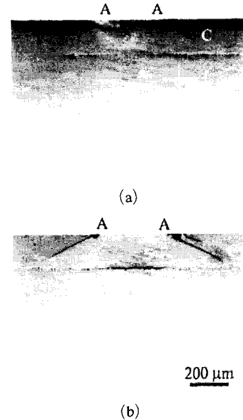
Fig. 5 Section views of contact damage in hard \text{Si}_3\text{N}_4 on soft \text{Si}_3\text{N}_4 with coating thickness d=180\ \mu\text{m} , showing (a) initiation at P=2000\ \text{N} and (b) propagation of contact cracks at P=3000\ \text{N} , using WC sphere radius r=1.98\ \text{mm} . Contact diameter AA indicated
