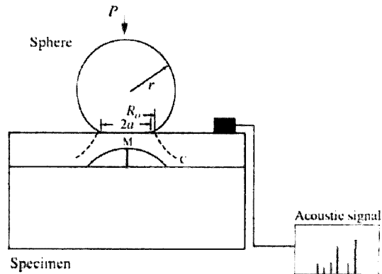
Fig. 1 Schematic diagram of contact tests. Typical cone crack (C) and transverse crack (M) are observed during contact with sphere indenter at load P . Tungsten carbide (WC) ball is indented on the flat surface. Contact radius a can be measured by optical microscope. Acoustic emission detector was attached on the flat surface of each specimen
