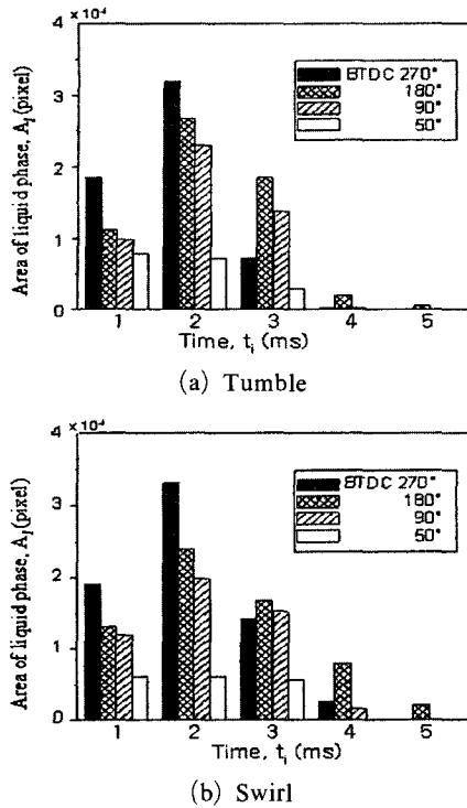
Fig. 4 Area occupied by liquid fuel
