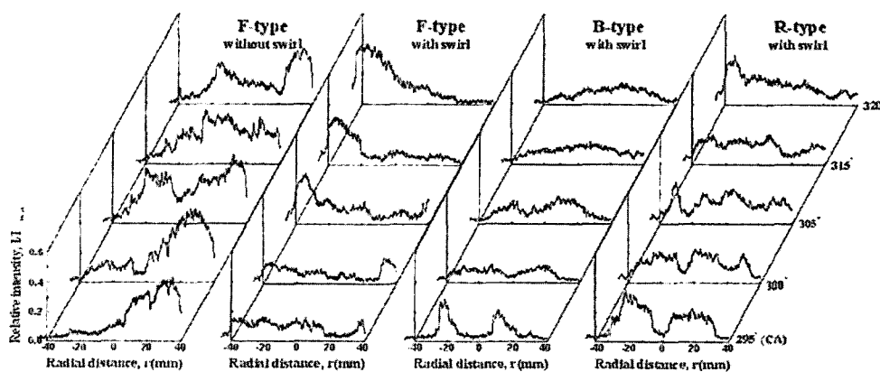
Fig. 9 Fluorescence intensity ratio profiles according to crank angle ( z=15 mm, SOI: 90° BTDC)
