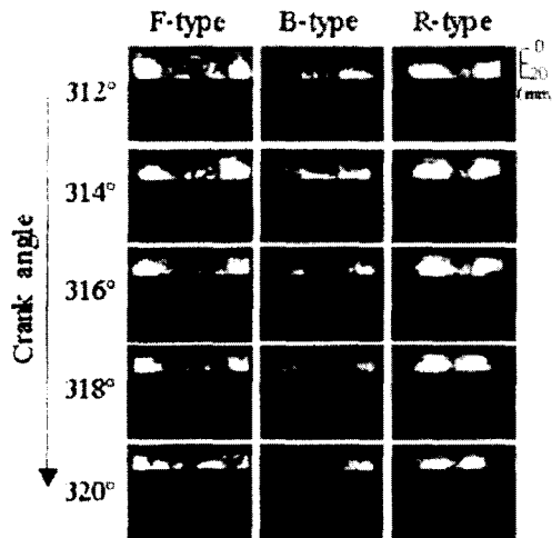
Fig. 10 Spray fluorescence images according to crank angle at injection timing of 60° BTDC
