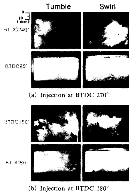
Fig. 6 Spray fluorescence images according to crank angle at early injection
