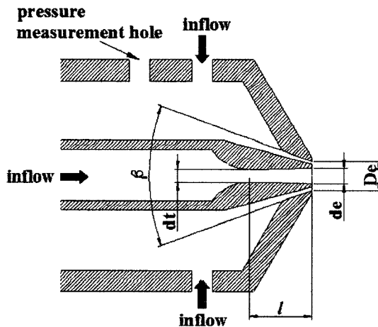
Fig. 2 Schematic of experimental coaxial nozzle.
