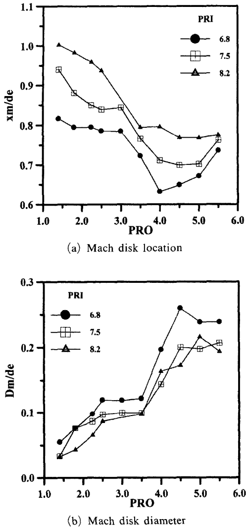
Fig. 10 Mach disk location and diameter vs. outer nozzle pressure ratio
