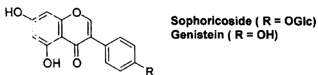
Fig. 1. Chemical structures of sophoricoside and genistein. Substituents are a glucose moiety (OGlc) and a hydroxyl group (OH).
