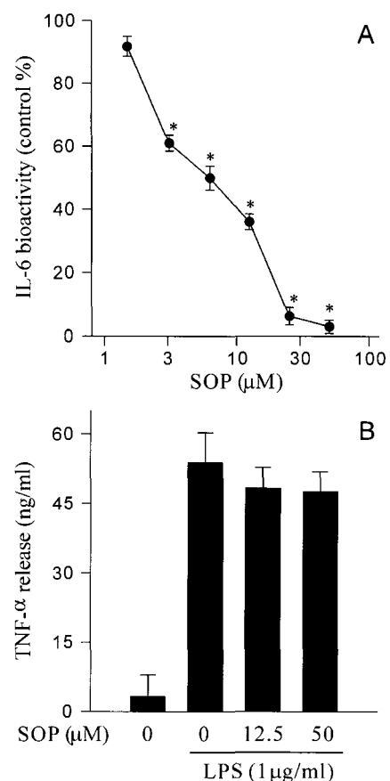
Fig. 2. Effects of sophoricoside on IL-6 bioactivity and TNF- \alpha release. Inhibitory effect of sophoricoside (SOP) on IL-6 bioactivity using hybridoma MH60/BSF-2 is represented as control %, mean \pm SEM of three independent tests assayed in triplicate (A). Significant difference from the control is p < 0.001 (*). Inhibitory effect of SOP on TNF- \alpha release in LPS-stimulated murine macrophages Raw264.7 was measured using an ELISA kit (B). Amount of TNF- \alpha released in the supernatant is represented as mean \pm SEM of three independent tests assayed in duplicate.
