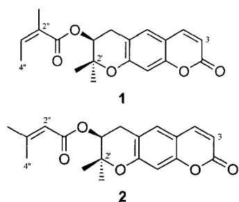
Fig. 1 Structures of compounds 1 and 2
