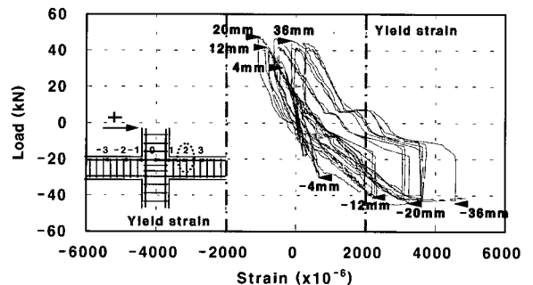
(f) Location 2 (model 4)
