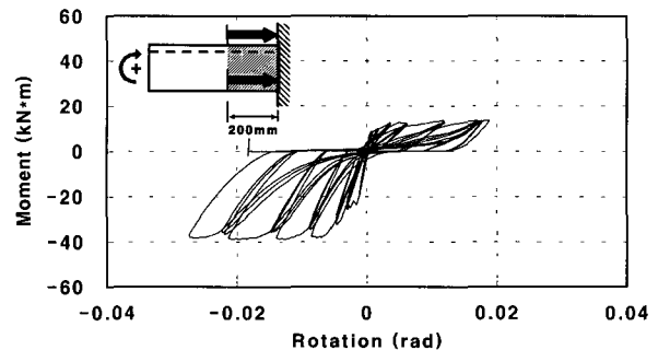
(c) Total rotation at plastic hinge region (model 4)
