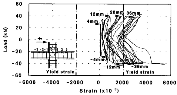
(a) Location 0 (model 3)
