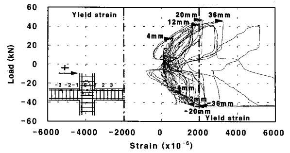
(b) Location 0 (model 4)
