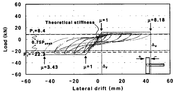
Fig. 9 Top drift-lateral load (model 5)
