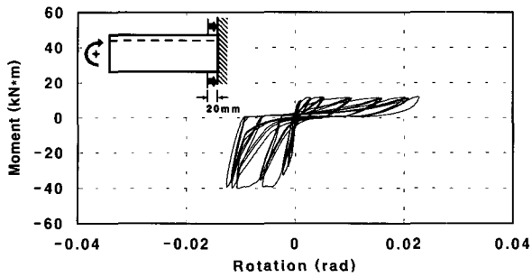
(a) Uplift rotation (model 3)
