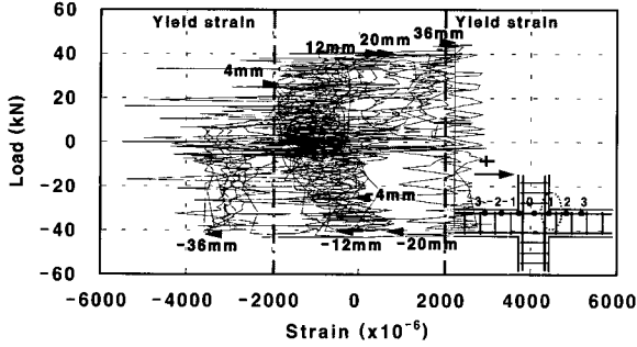
(c) Location 1 (model 3)
