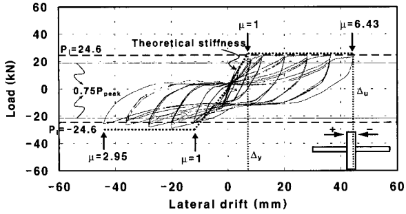
Fig. 5 Top drift-lateral load (model 1)
