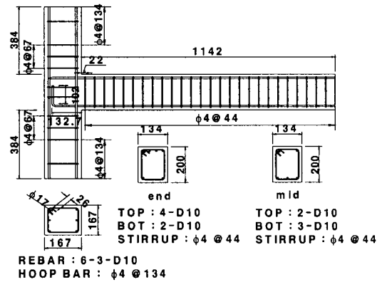
(a) Seismic details
