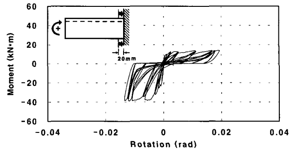
(a) Uplift rotation (model 4)
