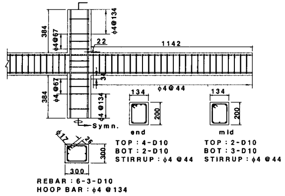
(a) Seismic details
