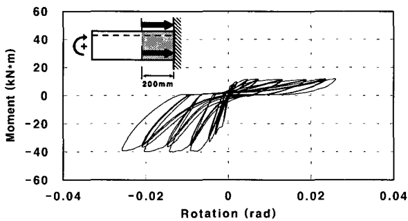
(c) Total rotation at plastic hinge region (model 3)
