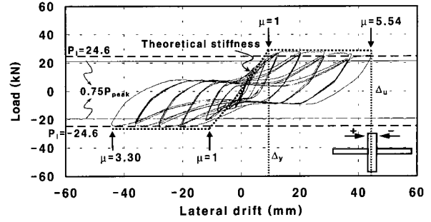
Fig. 6 Top drift-lateral load (model 2)
