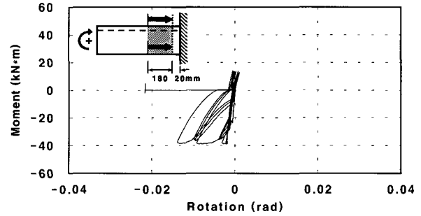
(b) Flexural rotation (model 4)
