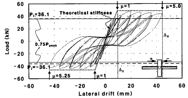
Fig. 8 Top drift-lateral load (model 4)
