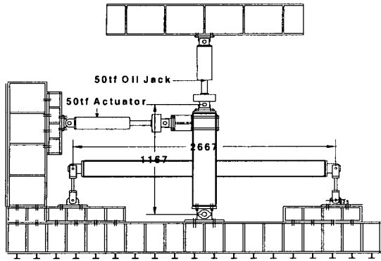
Fig. 4 Experimental setup (unit: mm)
