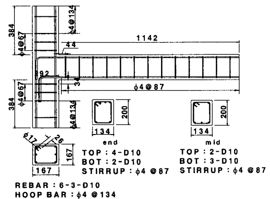
(b) Nonseismic details
