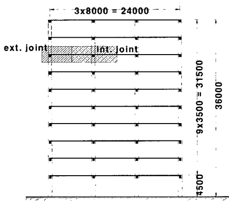
Fig. 1 Elevation of prototype structure (unit: mm)
