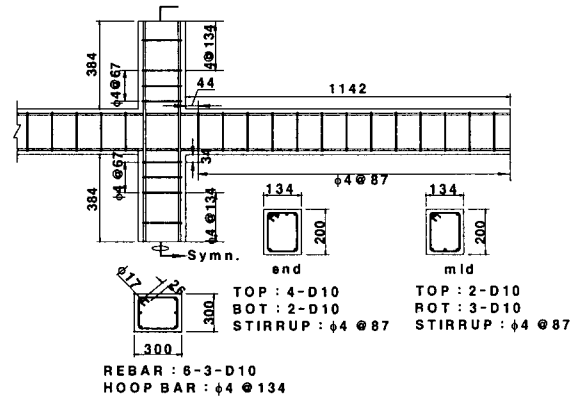
(b) Nonseismic details
