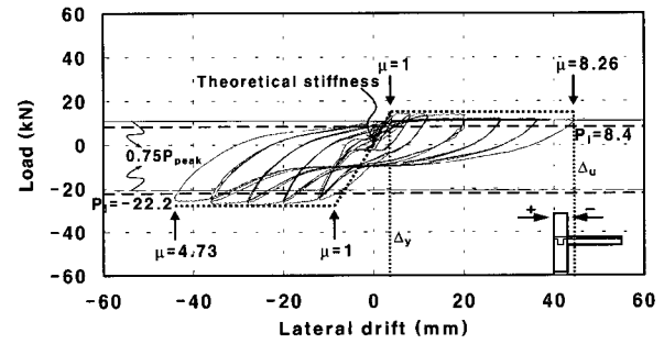
Fig. 10 Top drift-lateral load (model 6)
