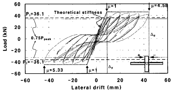
Fig. 7 Top drift-lateral load (model 3)
