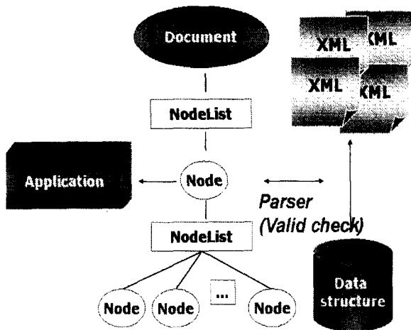
(Figure 5) DOM and Parser
