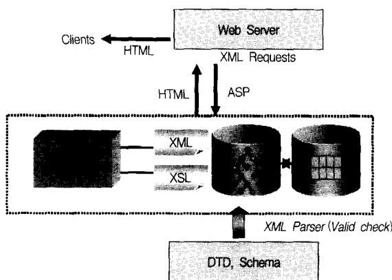
(Figure 3) XML Standard Technique and DataBase[10]
