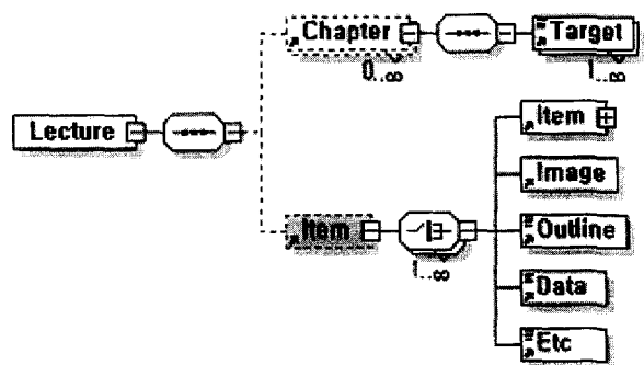
(Figure 11) Schema Modeling of the Data Operation
