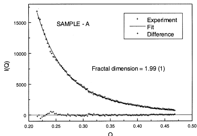
Fig. 4. SAXS data from sample A. Line is the fit to data ( \circ ) using equation 4 (see text). Also shown is the difference plot (+) between the data and fit.
