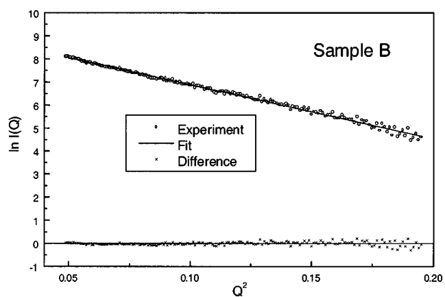
Fig. 5. SAXS data from sample B. Line is the fit to data ( \circ ) using cylindrical particles as a model using equation 3 (see text). Also shown is the difference plot (+) between the data and fit. The values for the cylinder radius and height are 7.8 Å and 21.8 Å respectively.
