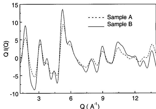
Fig. 2. The modified interference functions for the samples A (1000°C) and B (1900°C).
