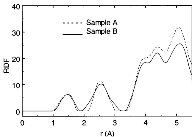
Fig. 3. The radial distribution functions for the samples A and B.
