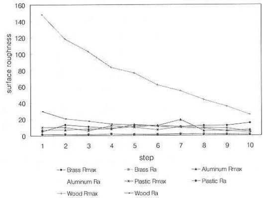
Fig. 5 Diagram of result by change the side-rake angle
