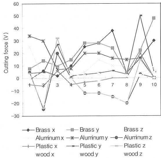
Fig. 5 Diagram of result by change the side-rake angle
