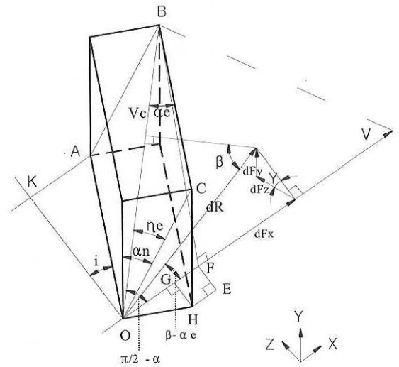
Fig. 2 Model by analysis of cutting force
