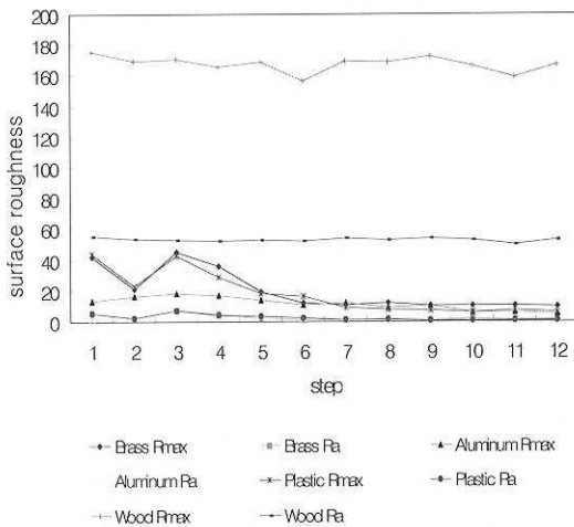
Fig. 4 Diagram of result by feedrate adjustment
