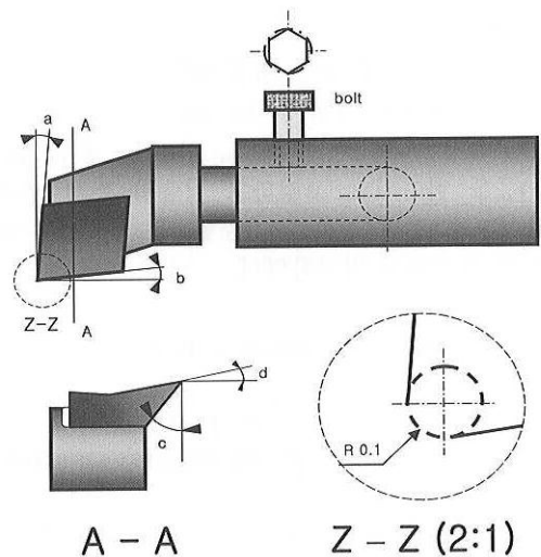
Fig. 3 Used bite shape and structure
