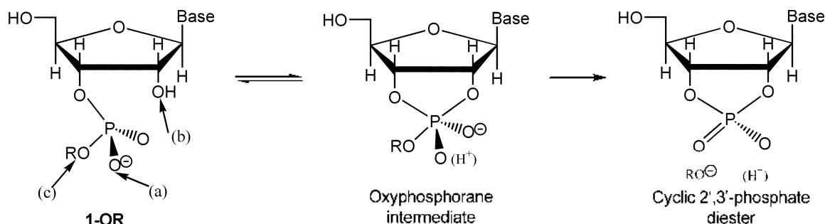
Scheme 1. The mechanism for cleavage of phosphate diesters.
