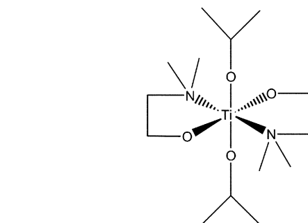
Figure 1. The proposed structure of the precursor [Ti(OPr) 2 (dmae) 2 ].
