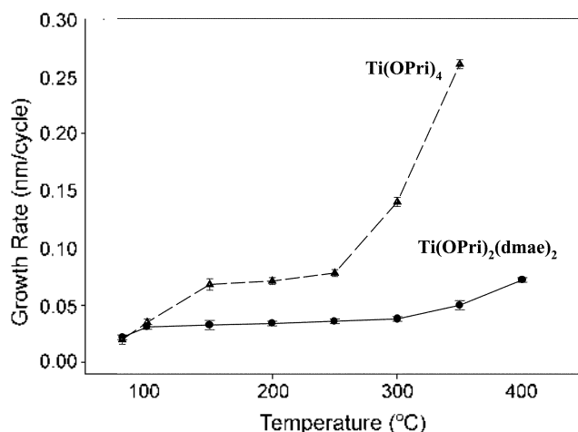
Figure 3. Temperature dependence of the growth rate for the \text{TiO}_2 films. The cycle consisted of 2 s exposure to [\text{Ti}(\text{OPr})_2(\text{dmae})_2] , 5 s Ar purge, 2 s exposure to water, and 5 s Ar purge.
