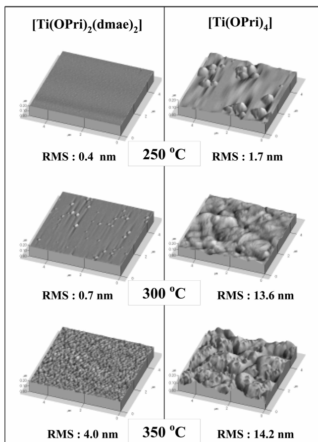
Figure 7. AFM images of \text{TiO}_2 films grown at 250–350 °C.
