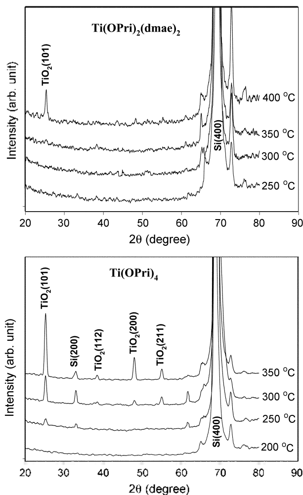
Figure 8. XRD patterns of \text{TiO}_2 films grown at 200–400 °C.
