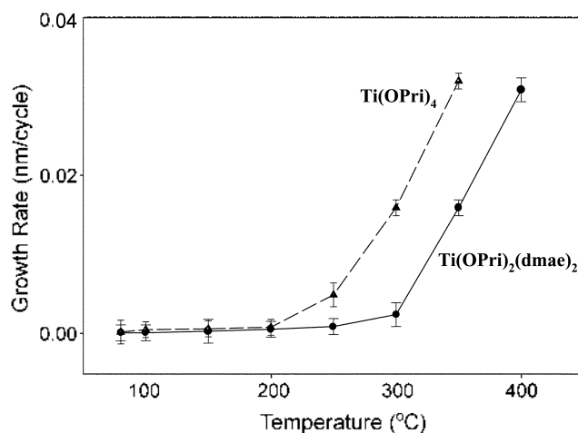
Figure 2. Temperature dependence of the growth rate for the \text{TiO}_2 films grown without water exposure. The cycle consisted of 2 s exposure to [\text{Ti}(\text{OPr})_2(\text{dmae})_2] , 5 s Ar purge, 2 s exposure to Ar, and 5 s Ar purge.
