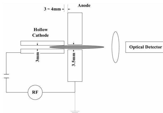
Figure 2. Geometric dimensions of the electrodes.
