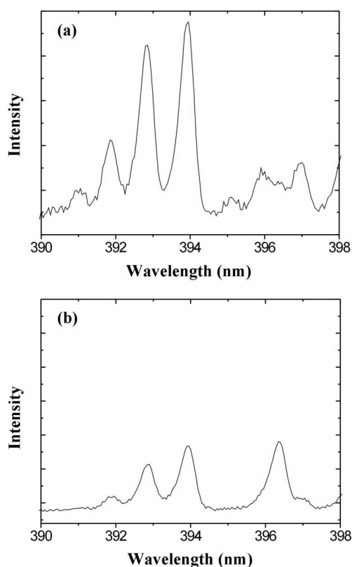
Figure 3. Emission spectra of H 2 S/Ar plasma powered by (a) RF or (b) AC.
