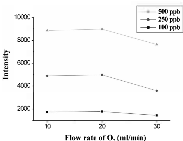
Figure 7. Effect of the flow rate of \text{O}_2 on \text{SO}_2^* emission line.
