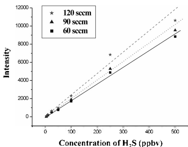
Figure 6. The plots of the \text{SO}_2^* emission line intensity vs. the sulfur concentration at various flow rates of the sample gas.
