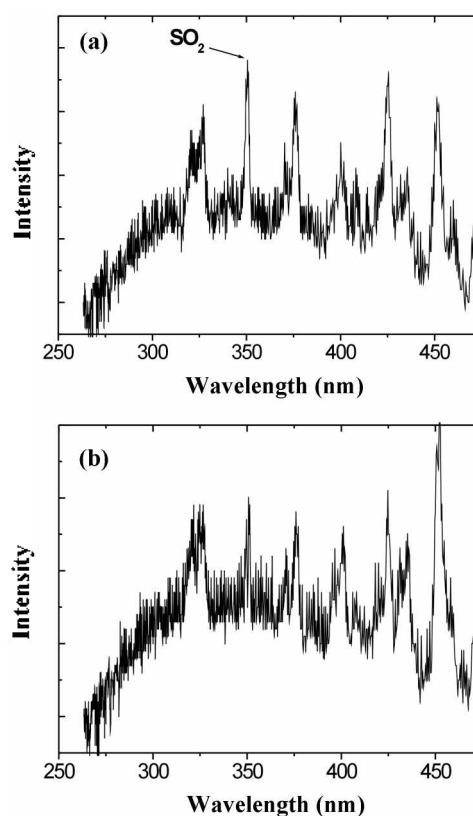
Figure 8. Emission spectra of (a) \text{SO}_2/\text{O}_2/\text{Ar} plasma and (b) \text{SO}_2/\text{Ar} plasma.
