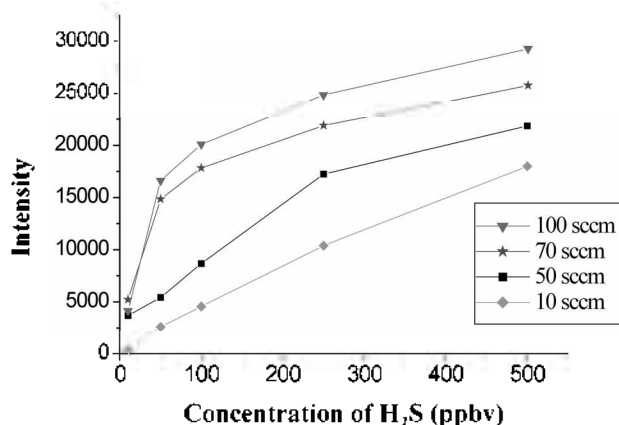
Figure 5. The plots of the \text{S}_2^* emission line intensity vs. the sulfur concentration at various flow rates of the sample gas (sccm, a unit of flow rate, equals to \text{mL min}^{-1} .)
