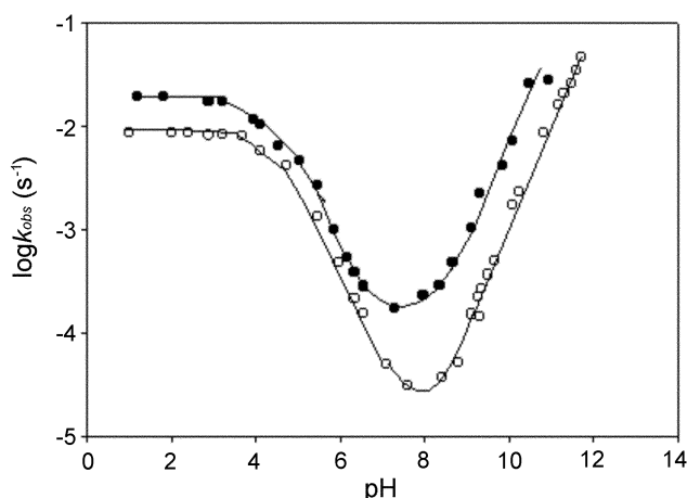
Figure 1. Plots of k_{\text{obs}} vs. pH for hydrolysis of N -benzoyl-4(5)-methylimidazole (●) and N -toluoyl-4(5)-methylimidazole (○) in \text{H}_2\text{O} at 25 °C and \mu = 0.5 M with KCl.
