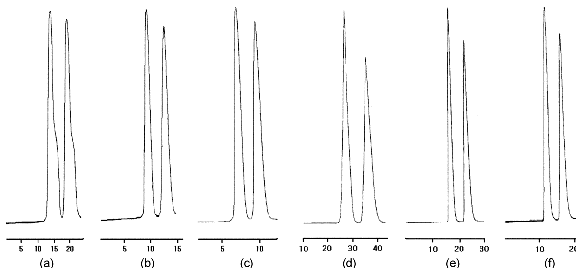
Figure 2. Chromatograms of the separation of racemic N -acetyl-1-naphthylethylamide ( 3 ) on preparative CSP 1 at different flow rates (F/R). Mobile phase: 20% 2-propanol in hexane. Sample injection volume (I/V): 0.2 mL (20 mg) (a) column size: 7.8 mm ID \times 250 mm length. F/R 4 mL/min. (b) F/R 6 mL/min. (c) F/R 8 mL/min. (d) column size: 10 mm ID \times 250 mm length. F/R 4 mL/min. (e) F/R 6 mL/min. (f) F/R 8 mL/min.
