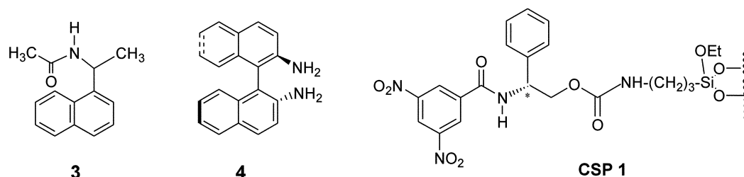
Figure 1. Structures of racemic samples ( N -acetyl-1-naphthylethylamide ( 3 ), 1,1'-binaphthyl-2,2'-diamine ( 4 )) and the chiral stationary phase (CSP 1 ) used in the study.
