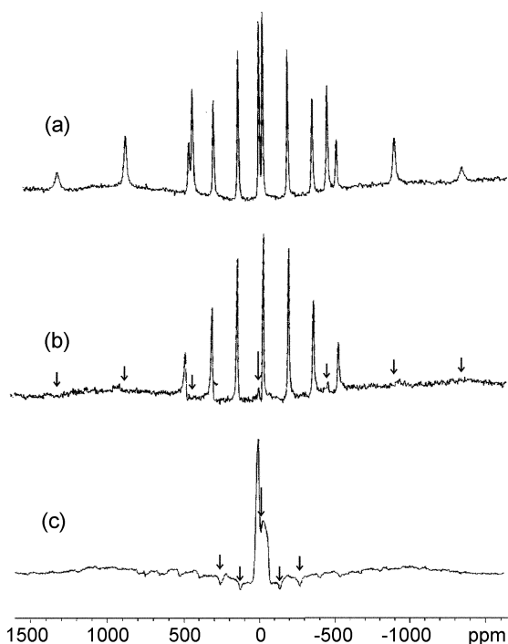
Figure 1. ^{133}\text{Cs} NMR spectra of \text{Cs}^+(15\text{-crown-5})_2\text{I}^- (a) non-selective irradiation with a single crystal (b) selective saturation with the single crystal (delay time of 42.4 \mu\text{s} ) and (c) selective saturation with a powder sample (delay time of 146 \mu\text{s} ). Irradiated peaks were indicated by arrows. The transmitter offset was indicated by longer arrows.
