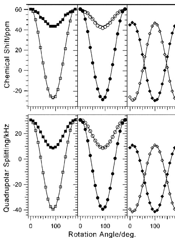
Figure 2. Single crystal ^{133}\text{Cs} NMR data of \text{Cs}^+(15\text{-crown-5})_2\text{I}^- and least-squares curves for the central transitions (upper) and quadrupolar splittings \nu_Q (lower) ( a axis; \square , \blacksquare , b axis; \circ , \bullet , c axis; \diamond , site1; solid symbol, site2; open symbol).
