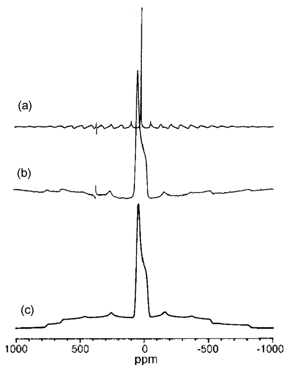
Figure 3. Powder ^{133}\text{Cs} NMR spectra of \text{Cs}^+(\text{15-crown-5})_2\Gamma^- (a) MAS (b) static (c) simulated spectrum with the single crystal data.
