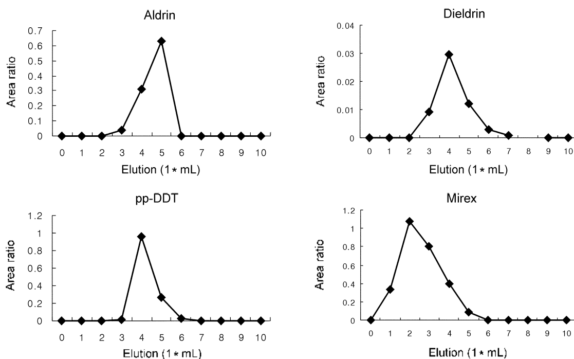
Figure 4. Elution patterns of aldrin, dieldrin, p,p-DDT and mirex through the silica gel-florisil column.
