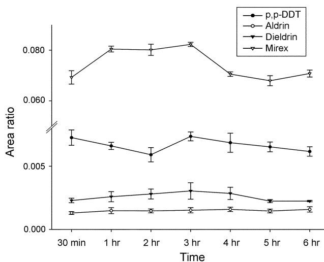
Figure 3. Comparison of extraction yields according to extraction time.
