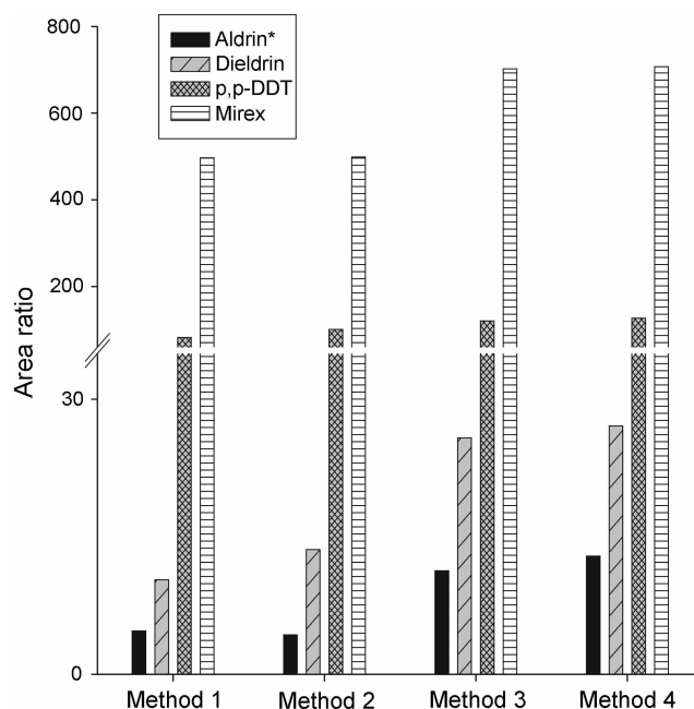
Figure 2. Comparison of extraction yields according to extraction methods used.
