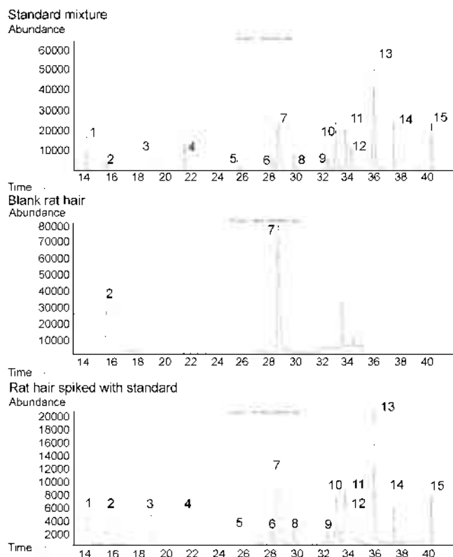
Figure 1. Chromatogram of standard mixture (20 ng/mL) and extract of sample spiked with POPs and ISTD on concentration of 20 ng/g. (1: hexachlorobenzene, 2: heptachlor, 3: aldrin, 4: heptachlor epoxide, 5: r -chloradane, 6: a -chloradane, 7: p,p-DDE, 8: dieldrin, 9: p,p-DDD, 10: endrin, 11: o,p-DDD, 12: o,p-DDT, 13: p,p-DDT, 14: mirex)
