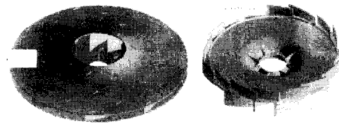
(a) Configuration of the impeller and diffuser
