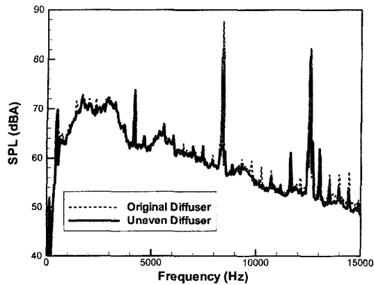
Fig. 11 Measured SPL for original and uneven pitched diffusers. (SPLs at BPF, 2 nd and 3 rd harmonic frequencies of original diffuser and uneven diffuser are 70.2, 87.3, 81.8, 73.3, 83.7, 81.2 dB(A), respectively)
