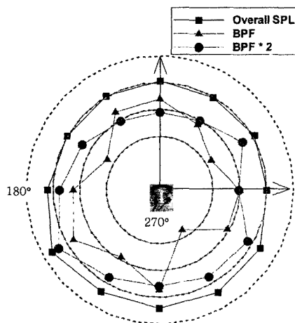
Fig. 5 Directivity pattern of centrifugal fan
