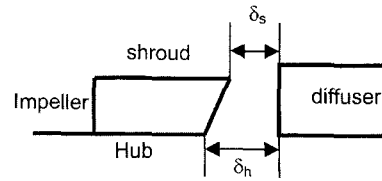
Fig. 12 Schematic diagram of new tapered impeller
