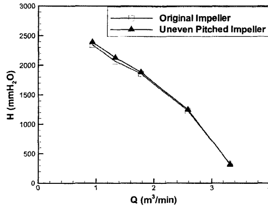
Fig. 8 Performance for original and uneven pitched impeller
