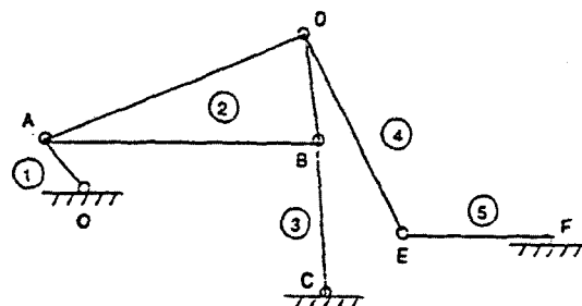
Fig. 3(a) Schematic view of a mechanism
