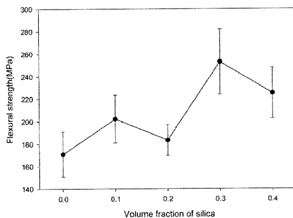
Figure 8. Flexural strength of EMC (65 vol% of fillers) function of the composition of the silica in the binary filler sy-
