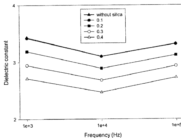
Figure 6. Dielectric constant of EMC (65 vol% of fillers) as a function of frequency with varying the composition of the silica in the binary filler system.
