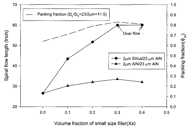
Figure 4. Spiral flow length of EMC (65 vol% of fillers) as a function of the composition of the small size filler in the binary filler systems.
