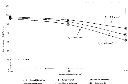
Fig. 9 The relationship between film thickness and dimensionless radius
