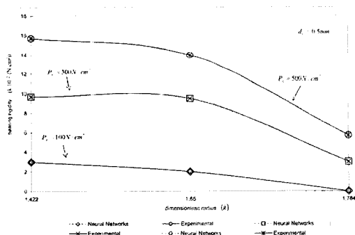
Fig. 8 The relationship between bearing rigidity and dimensionless radius
