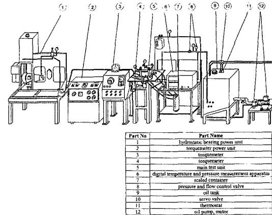
Fig. 2 The schematic experimental setup
