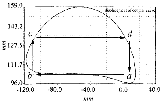
Fig. 5 Coupler trajectory
