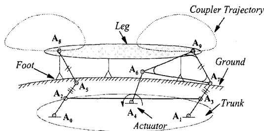
Fig. 4 Kinematic design of leg
