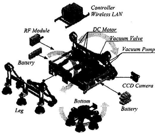
Fig. 6 System layout
