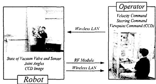
Fig. 11 Experimental setup
