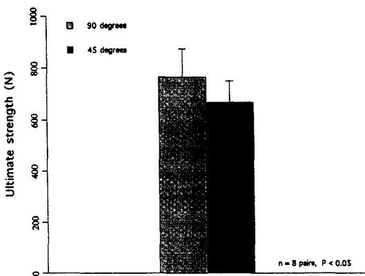
Fig. 3(b) Ultimate load of the bone-tendon specimens at different degrees of loading. Statistical analysis (Two-way ANOVA test) revealed that a significant difference in ultimate load was found between 45° and 90° of loading ( p < 0.05 )
