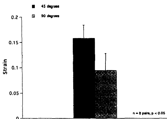
Fig. 5 Comparison of the failure strains of the bone-tendon junction at the ultimate load in tensile tests. The largest failure strain occurred at 45°, being 1.7 times the failure strain at 90°
