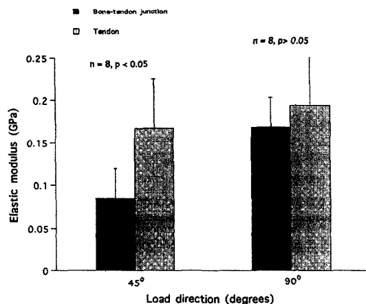
Fig. 7 Elastic modulus representing initial linear part of slope of stress-strain curve were measured for tendon and bone-tendon junction at 45° and 90° of loading. A significant difference in elastic modulus was noted using a two-way ANOVA for tendon and the bone-tendon junction at 45° ( p < 0.05 ). But no significant difference was found between tendon and bone-tendon junction at 90° ( p > 0.05 )
