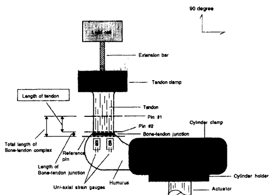
Fig. 1 Sketch shows the bone-tendon specimen during a tensile test
