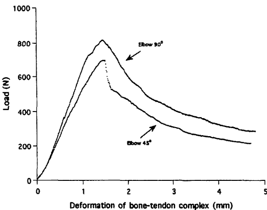
Fig. 3(a) Typical load vs deformation curves of load to failure tests of bone-tendon specimens at different degrees of elbow flexion
