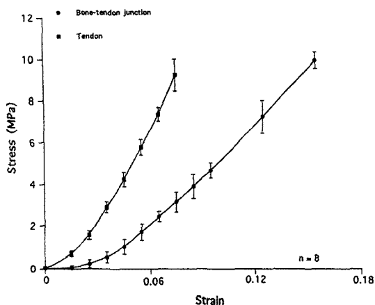
Fig. 4 Engineering stress-strain curves of tendon and bone-tendon junction at 45° of loading. Statistical analysis (Two-way ANOVA test) revealed that there are significant differences in strains of tendon and bone-tendon junction ( p < 0.05 )
