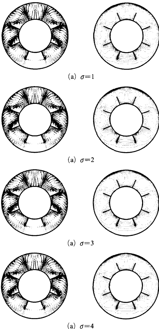
Fig. 13 Velocity vectors and isotherms for the different values of \sigma=1\sim 4 at Ra=10^5
