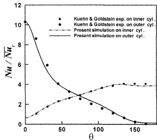
Fig. 3 Comparison of the local Nusselt number at the inner and outer cylinder walls as a function of \theta with experimental results when \sigma=0.625 and Ra=4.7 \times 10^4
